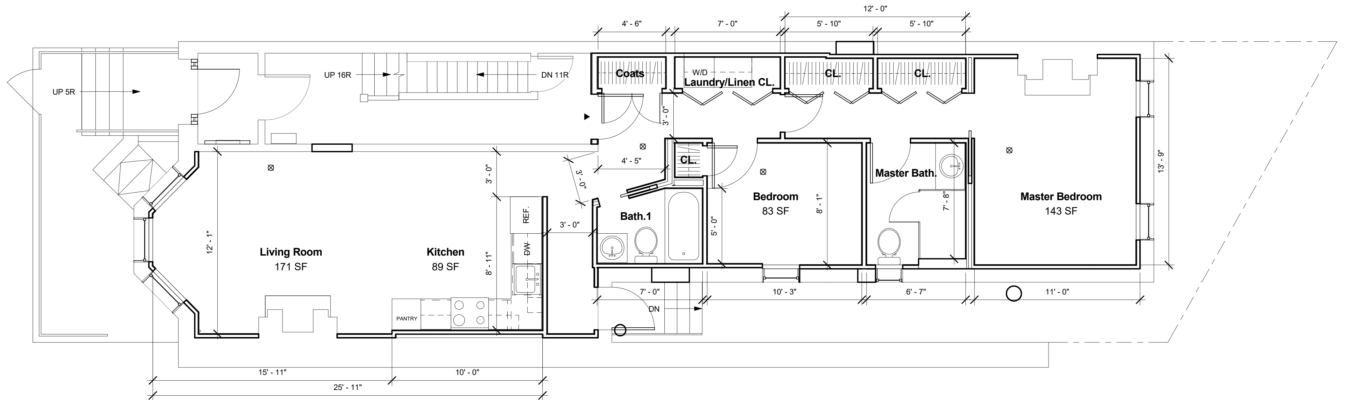
① 1st Floor Plan 1/4" = 1'-0"
