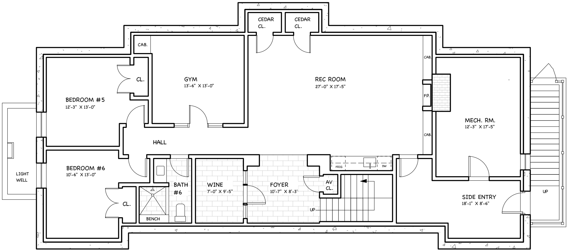
○ BASEMENT PLAN
