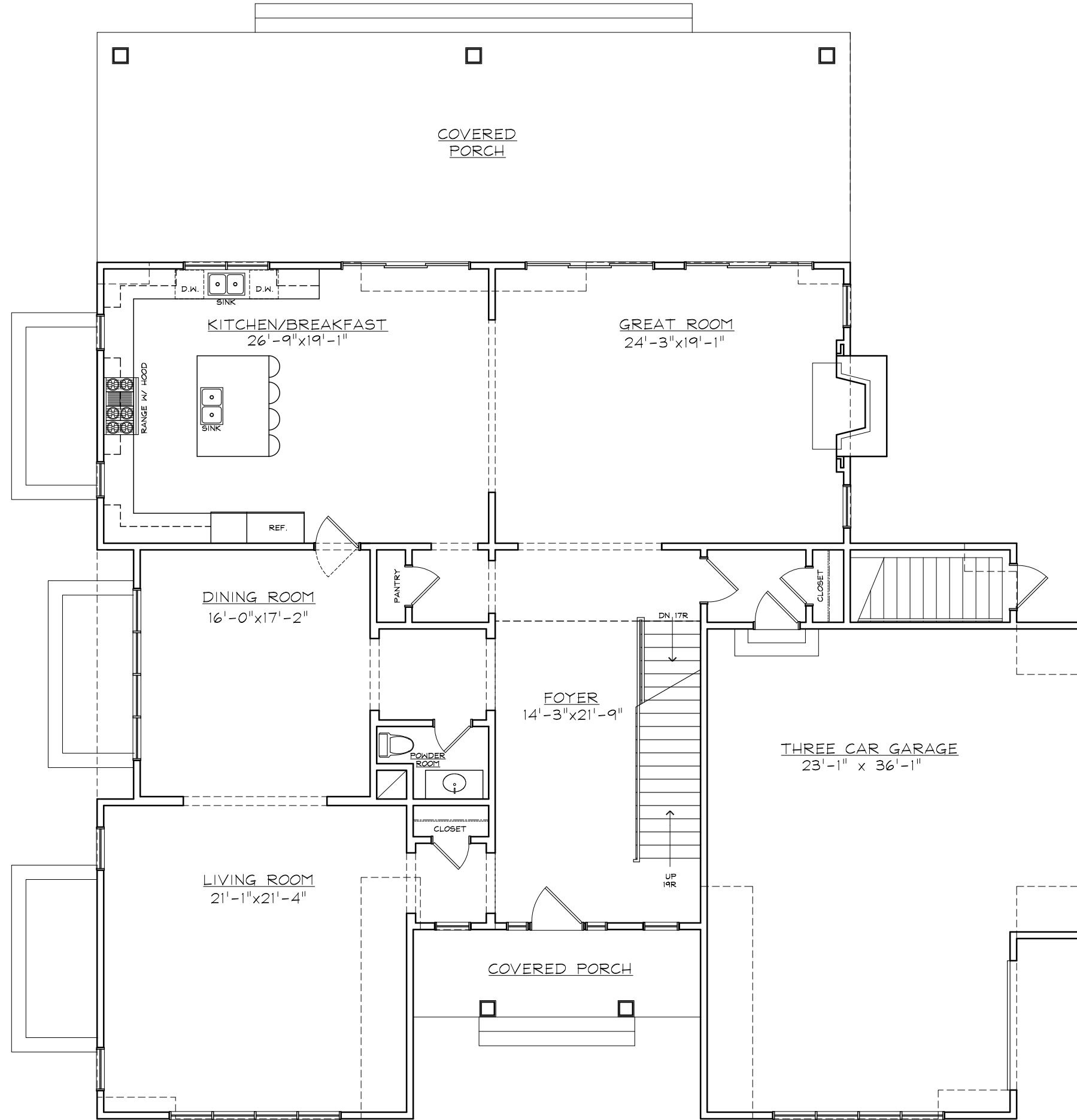
FIRST FLOOR PLAN DEERFIELD LOT 2
