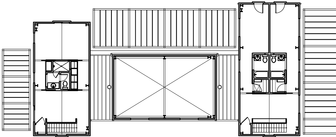
STEEL HOUSE SECOND FLOOR
