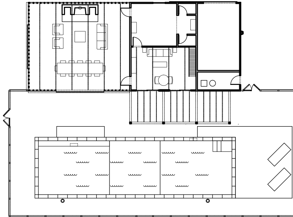
POOL HOUSE FIRST FLOOR
