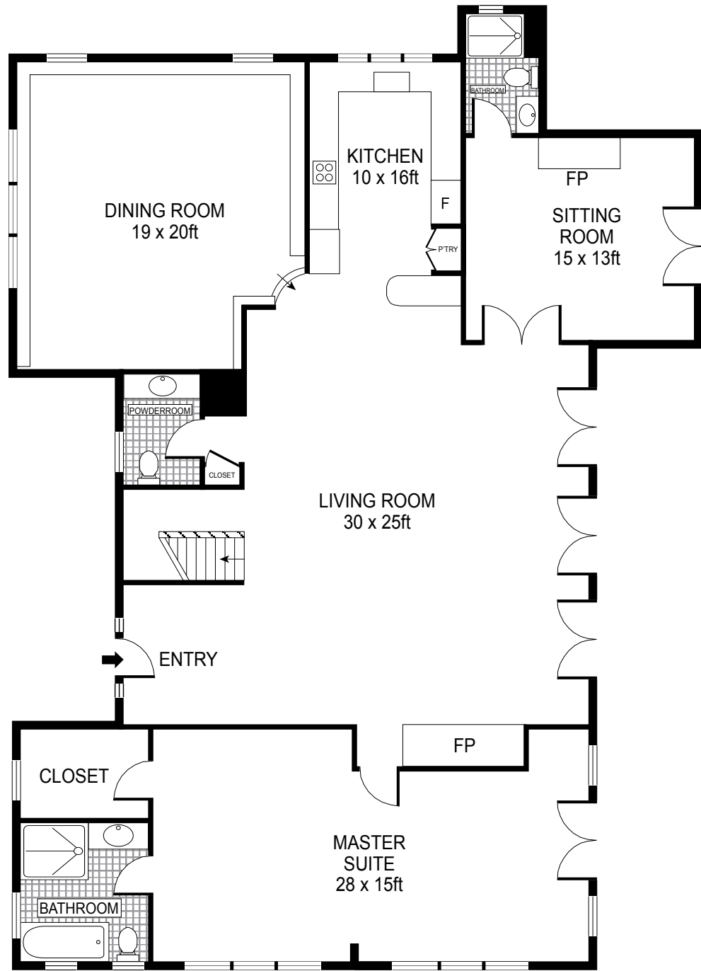
FIRST FLOOR
