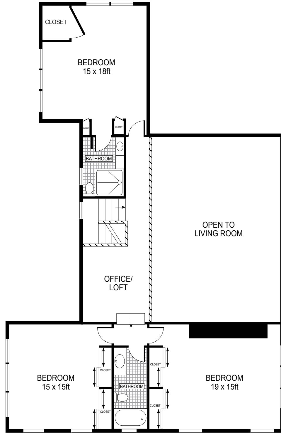
SECOND FLOOR
