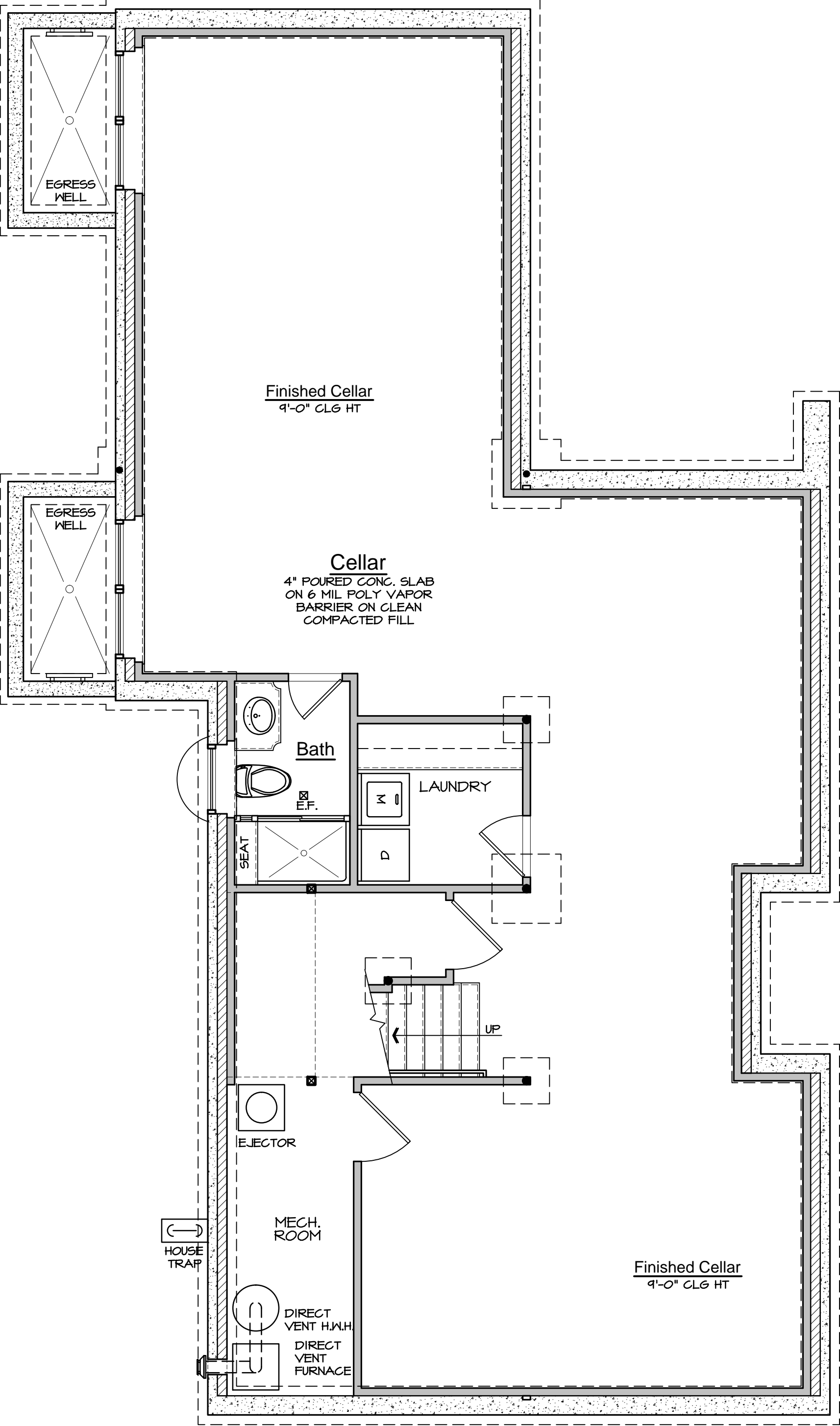
Cellar Plan
