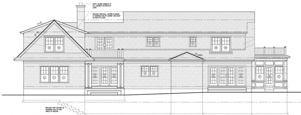
1 PROPOSED REAR ELEVATION
