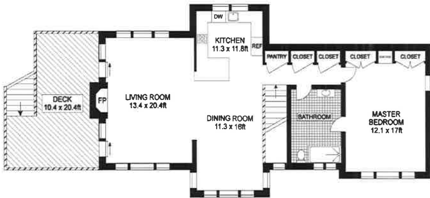
SECOND FLOOR
