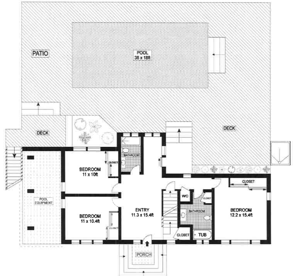
FIRST FLOOR
