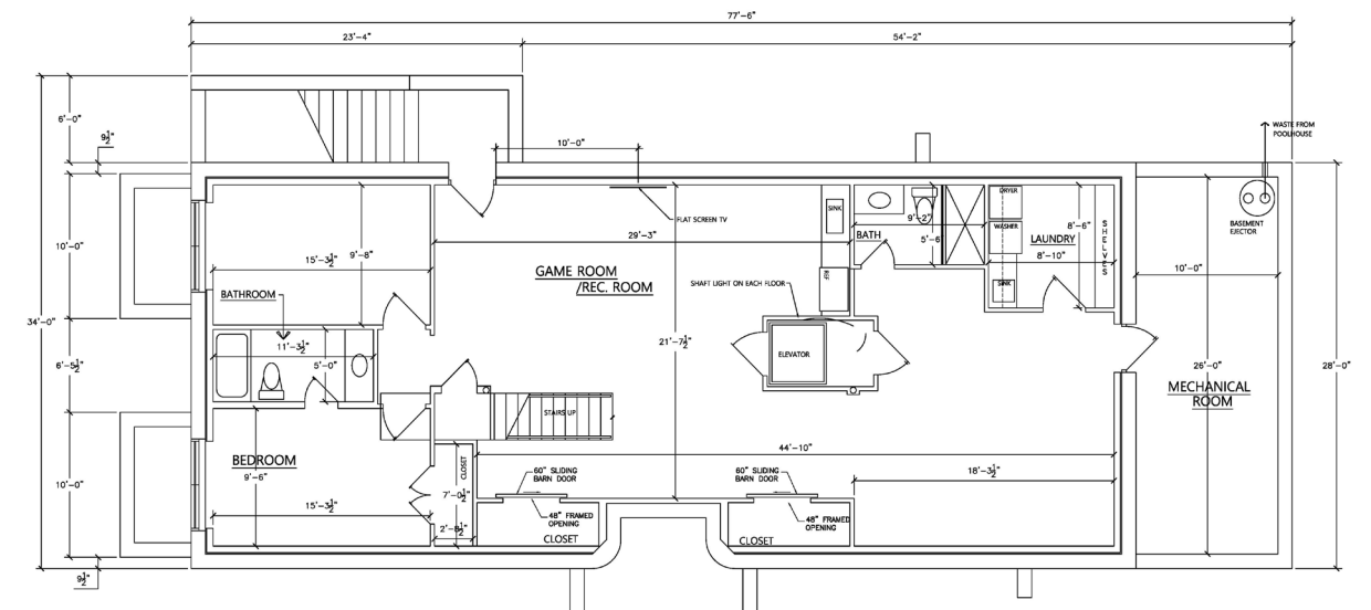
Finished Basement Plan
