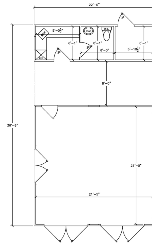
Garage & Pool House Plan
