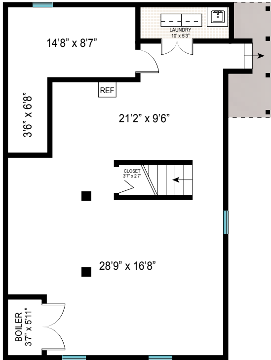
BASEMENT
