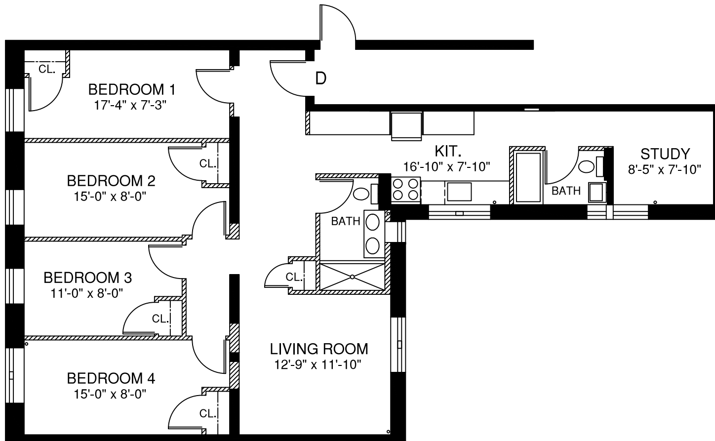
PROPOSED FLOOR PLAN Scale: 1/8" = 1'-0"
