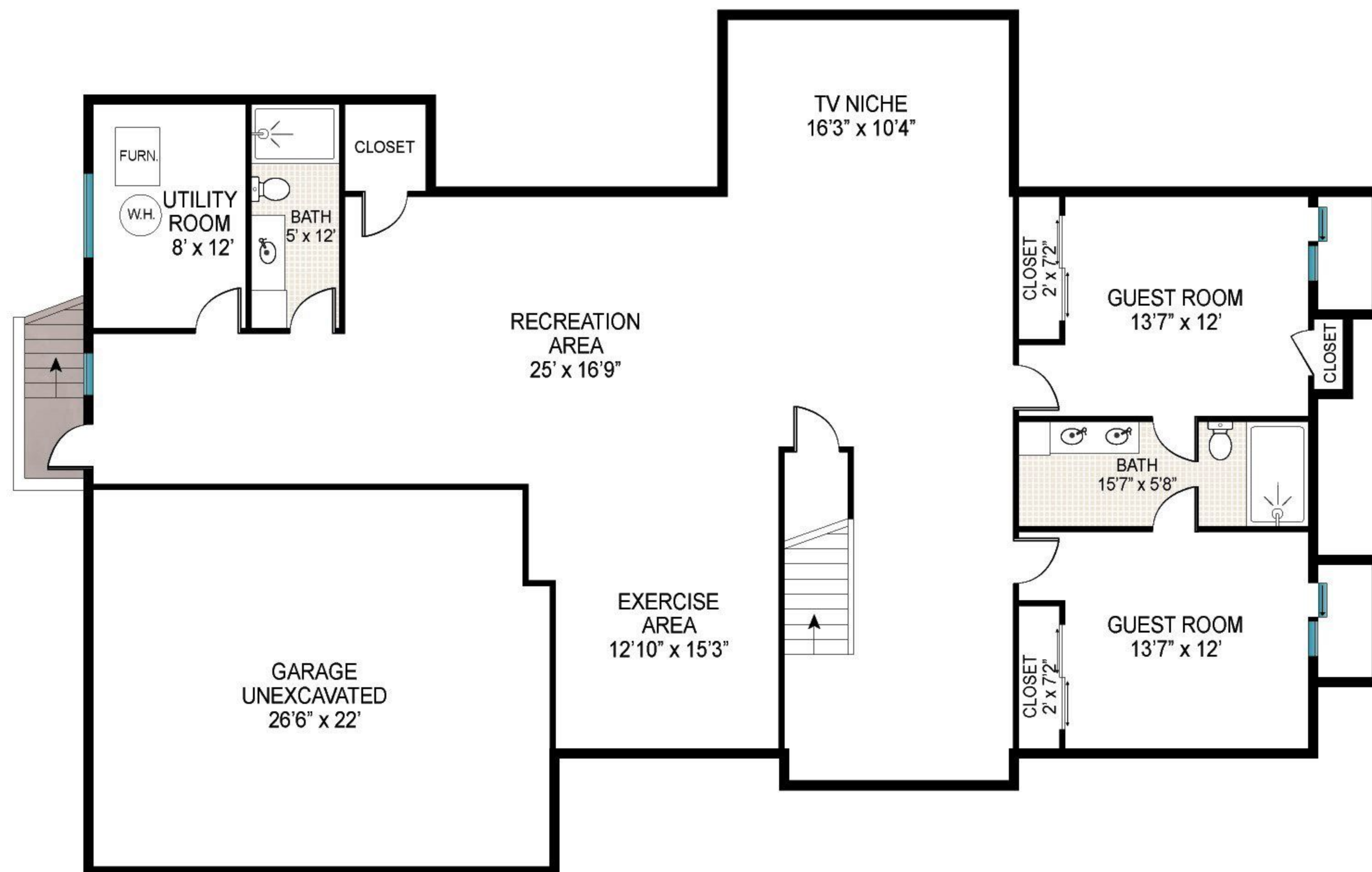
BASEMENT
