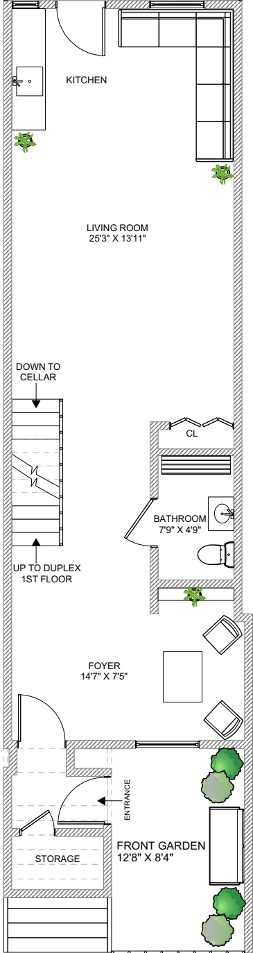
GARDEN FL / DUPLEX 1ST LEVEL
