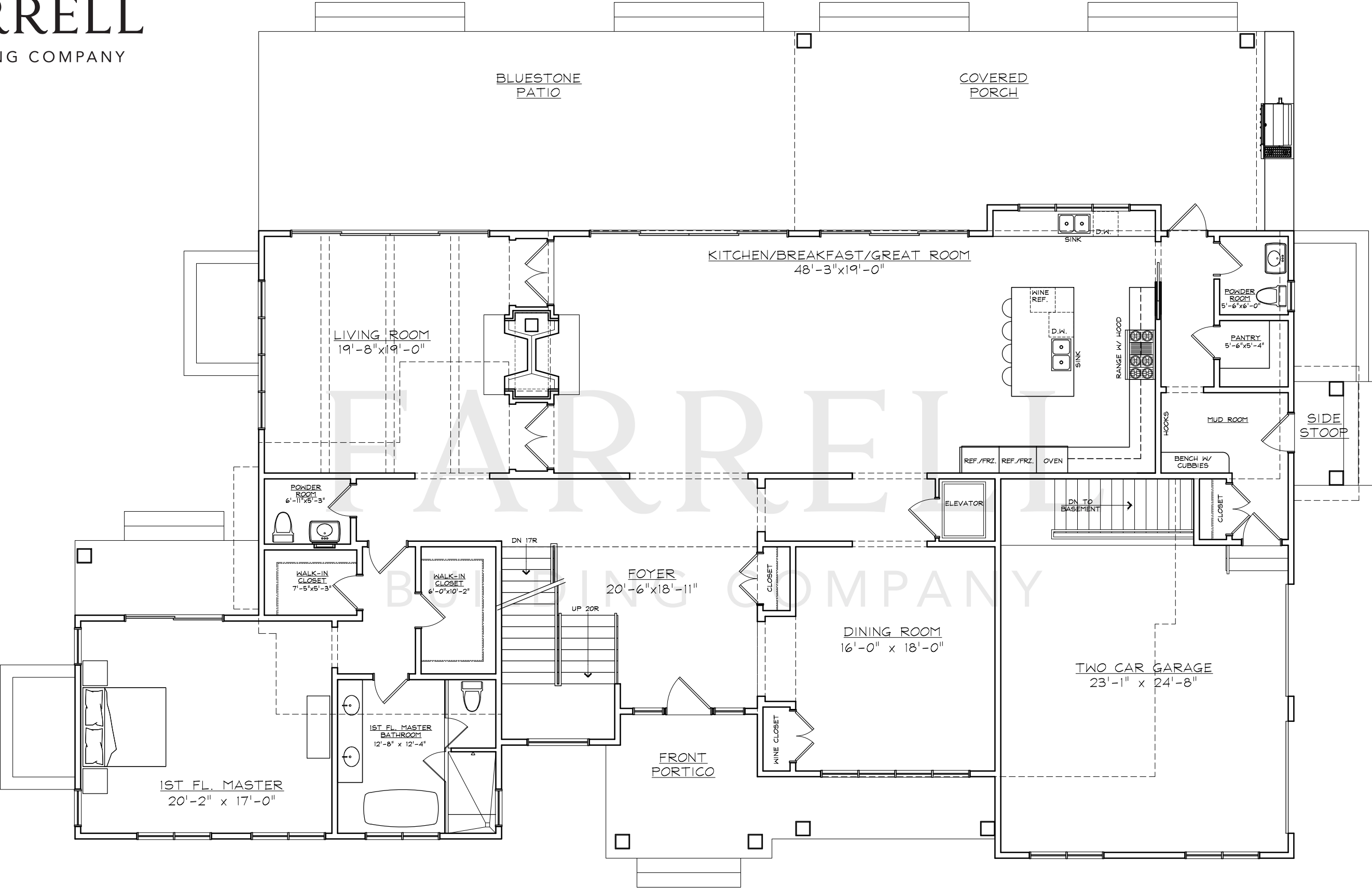
FIRST FLOOR PLAN (03-01-18) 193 / 215 MECOX ROAD 3,435 SQ. FT. TOTAL 6,064 SQ. FT.
