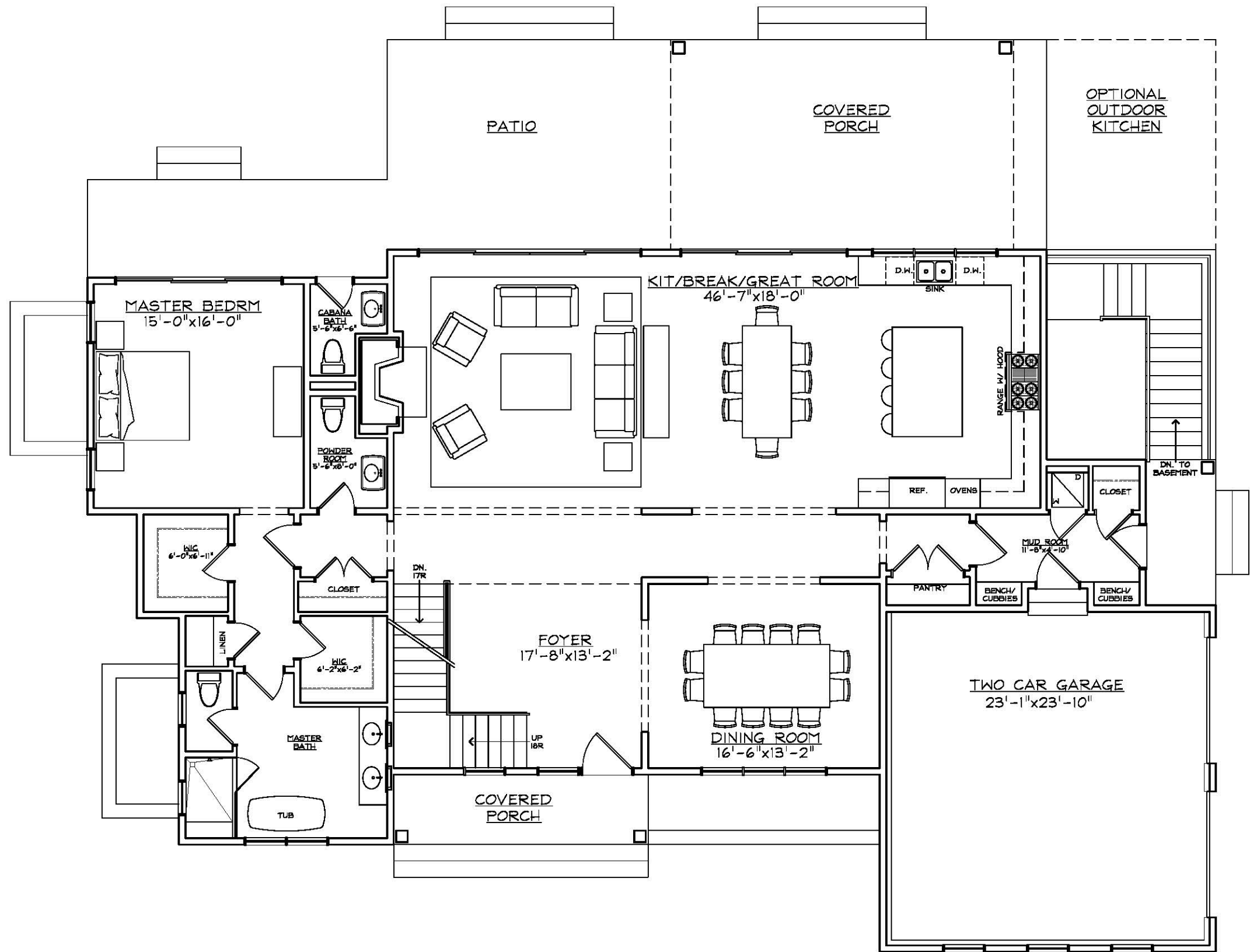
FIRST FLOOR PLAN (09-29-17) 10 SAGG ROAD
