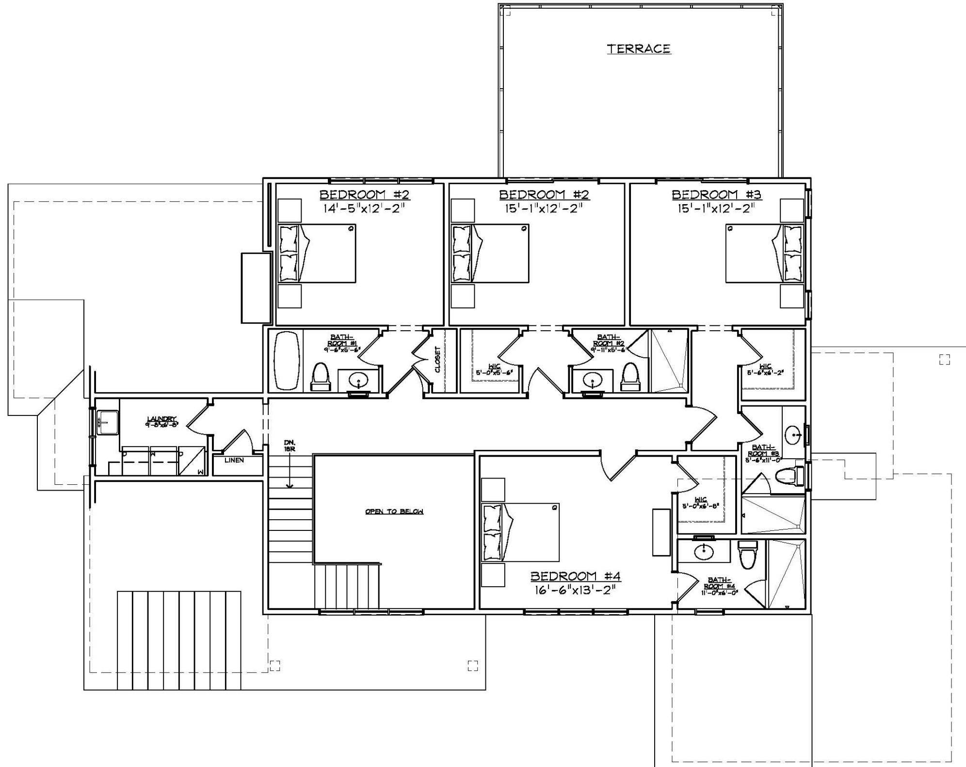
SECOND FLOOR PLAN (09-28-17) 10 SAGG ROAD
