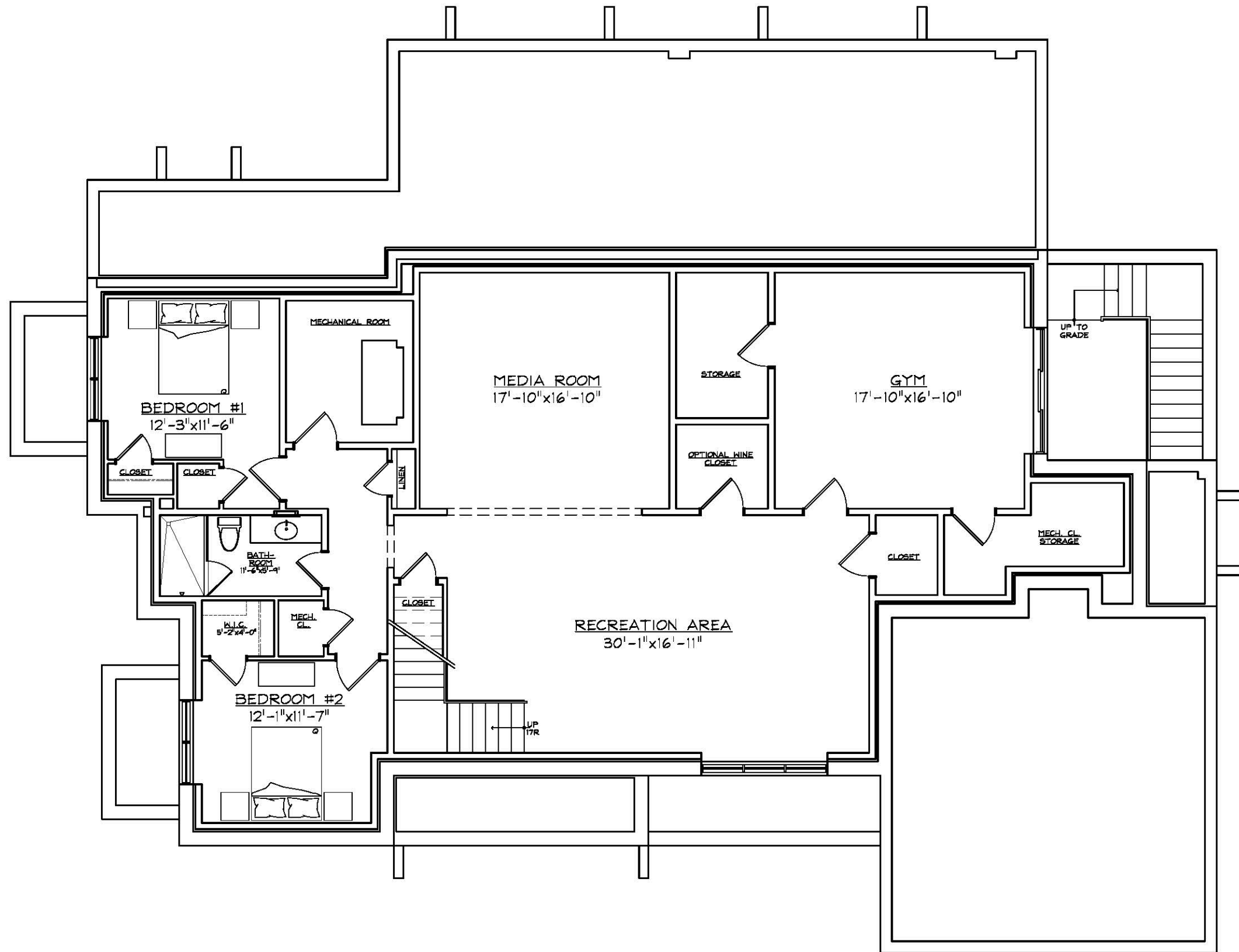
BASEMENT PLAN (09-29-17) 10 SAGG ROAD
