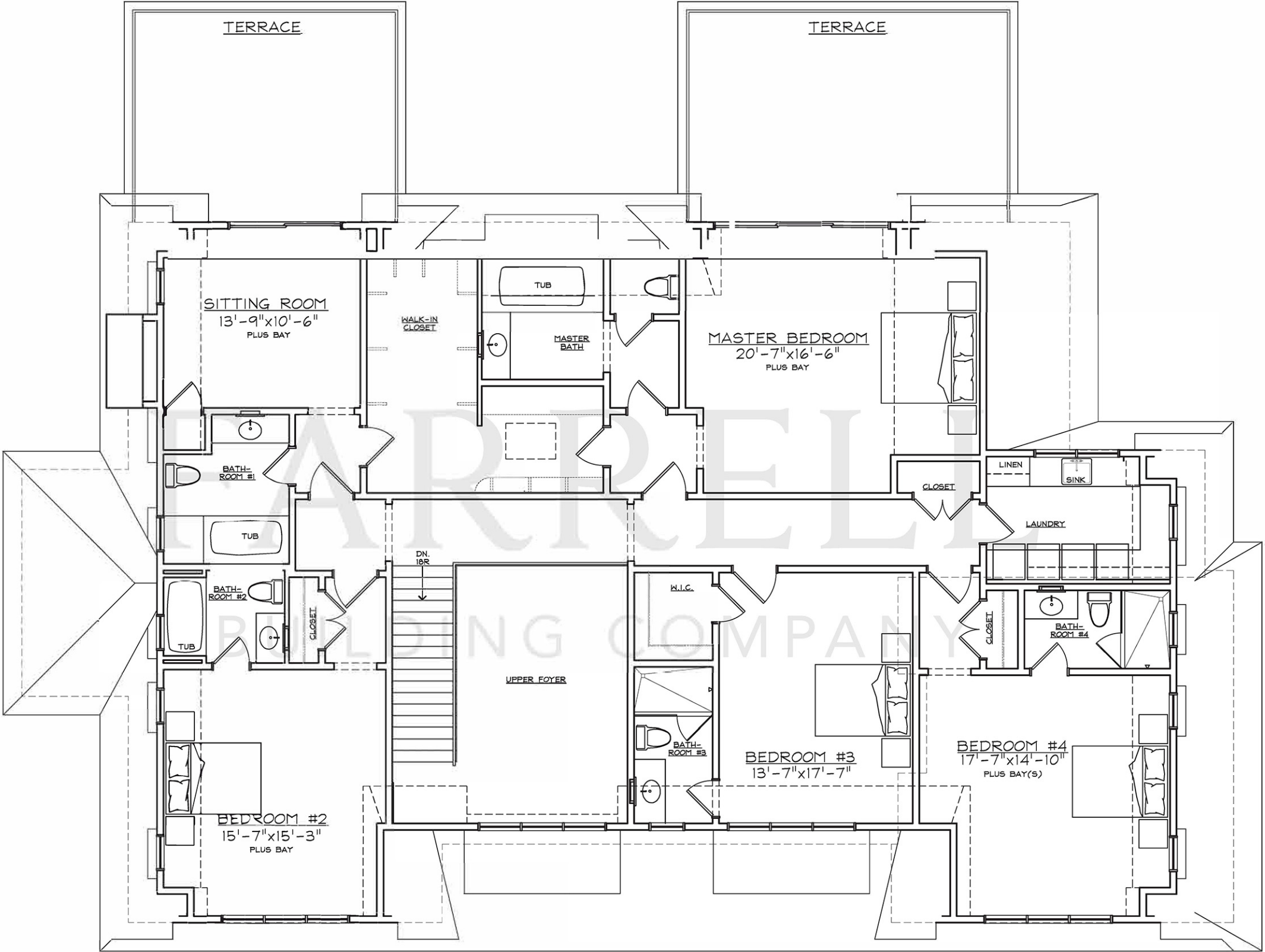
SECOND FLOOR PLAN (06-15-18) 30 LAWRENCE COURT 2,670 SQ.FT.
