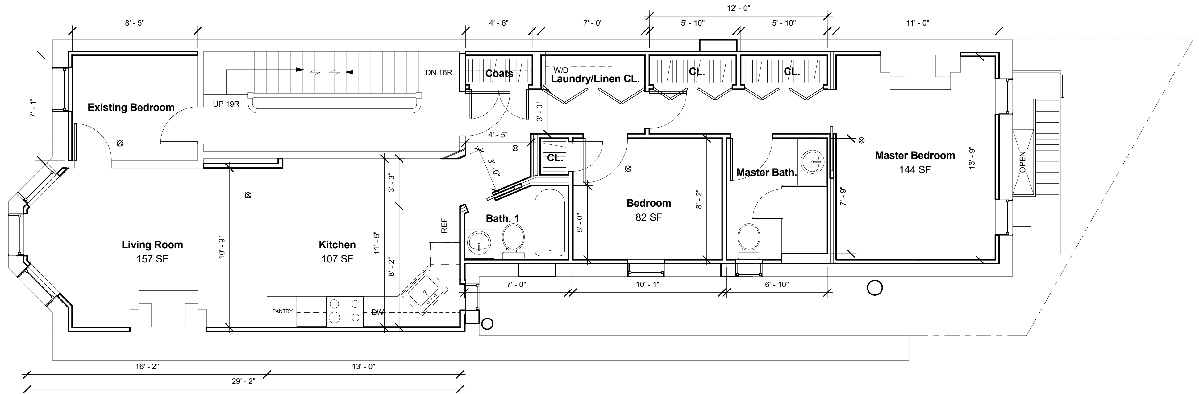
① 3rd Floor Plan 1/4" = 1'-0"
