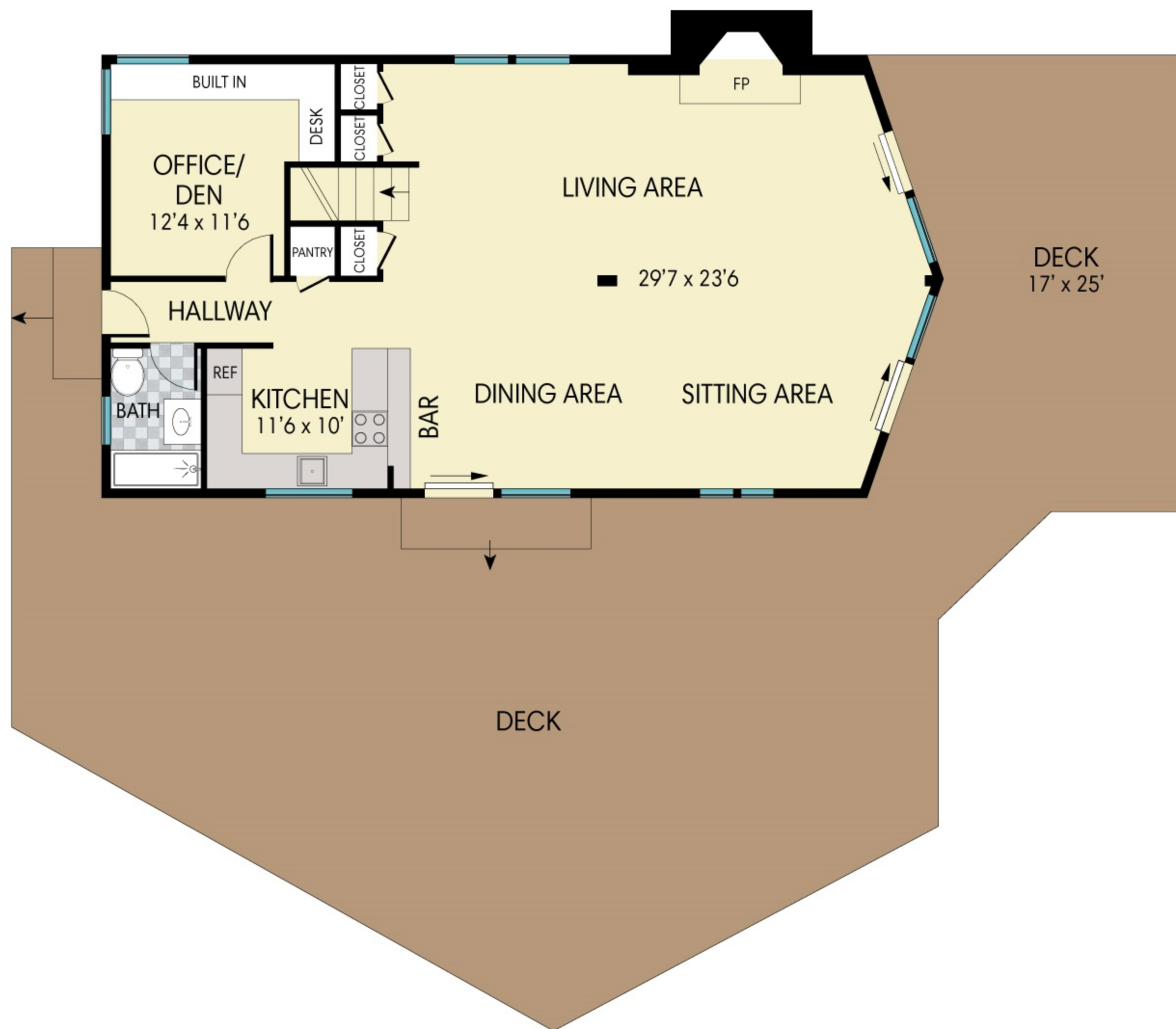
FIRST FLOOR
