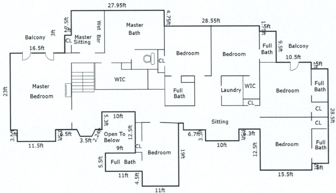
Second Floor [3322.63 Sq ft]
