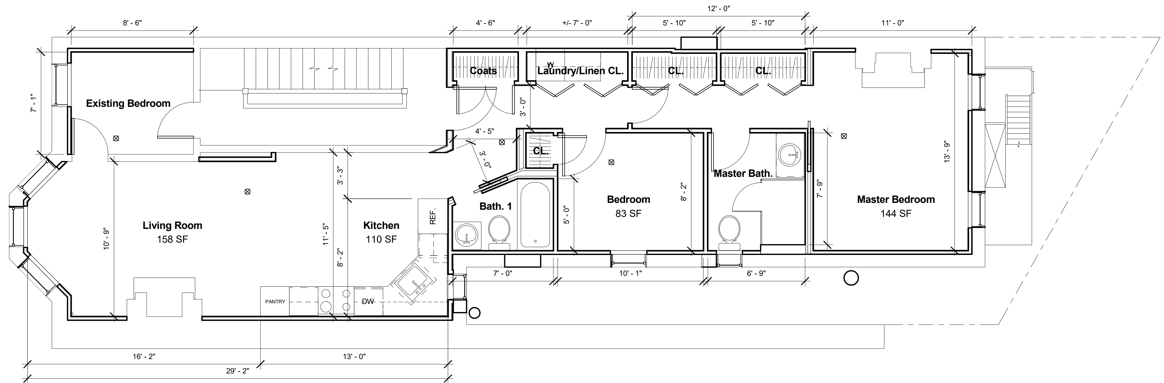
① 2nd Floor Plan 1/4" = 1'-0"
