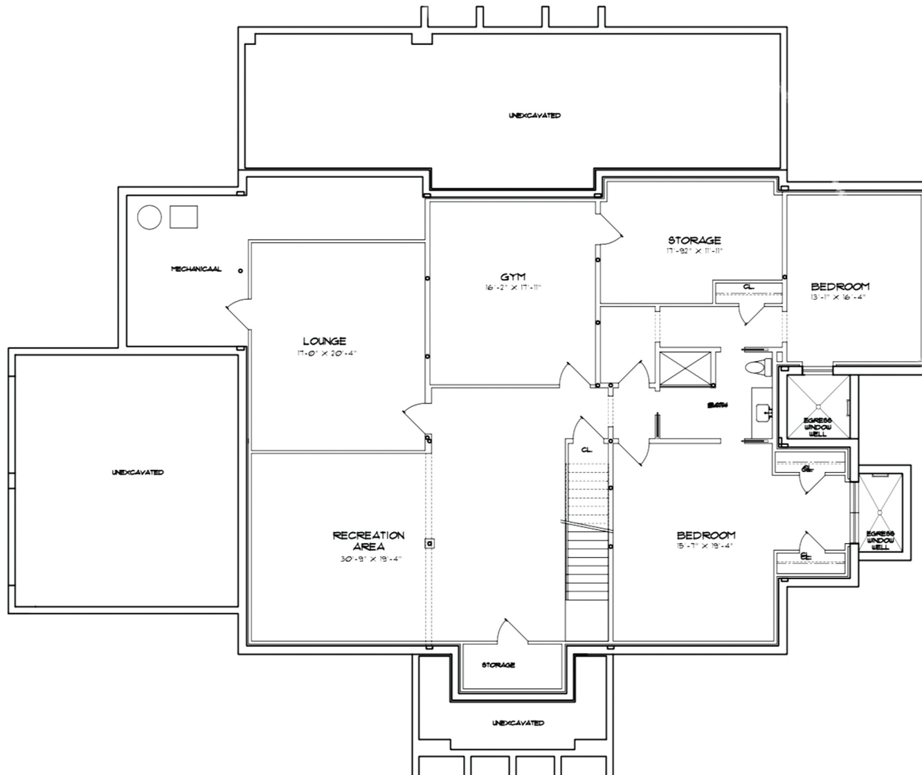
FINISHED BASEMENT PLAN 1390 S.F.
