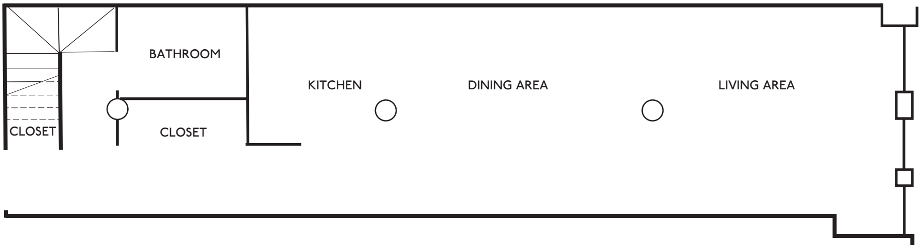
1 MAIN FLOOR: FLOOR PLAN 55' x 12'6"
