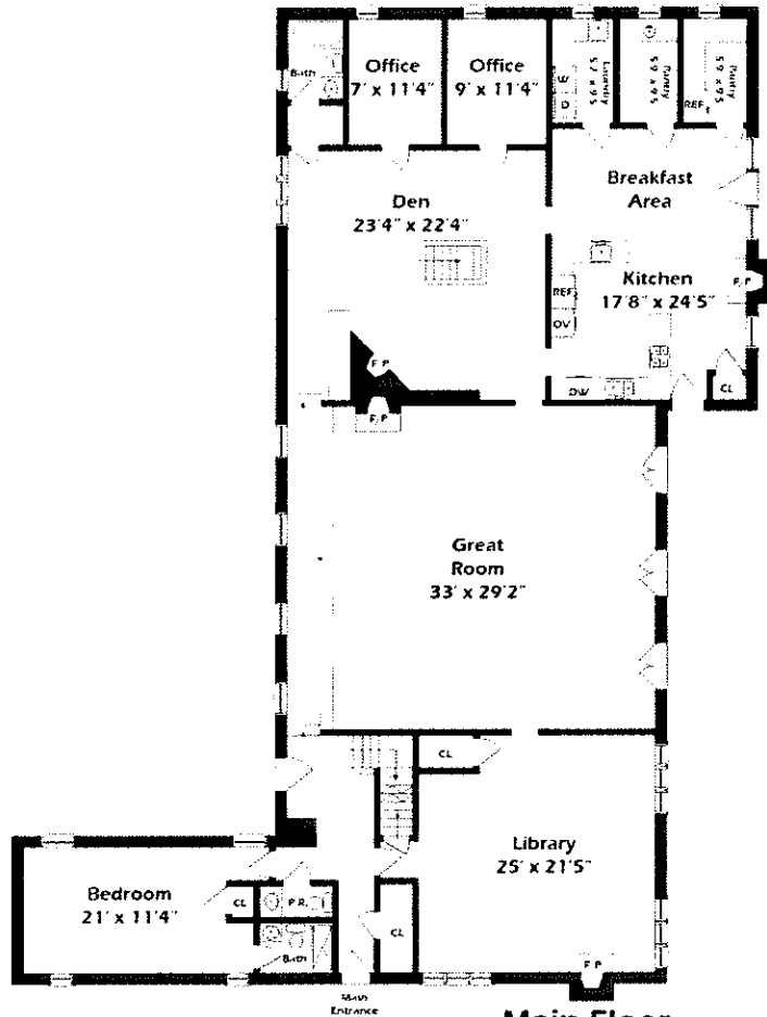
Main Floor
