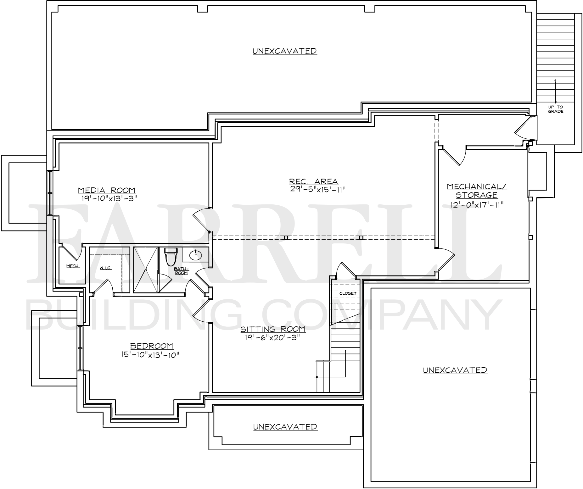
LOWER LEVEL PLAN (03-17-16) ROSES GROVE ROAD 1,922 SQ.FT.
