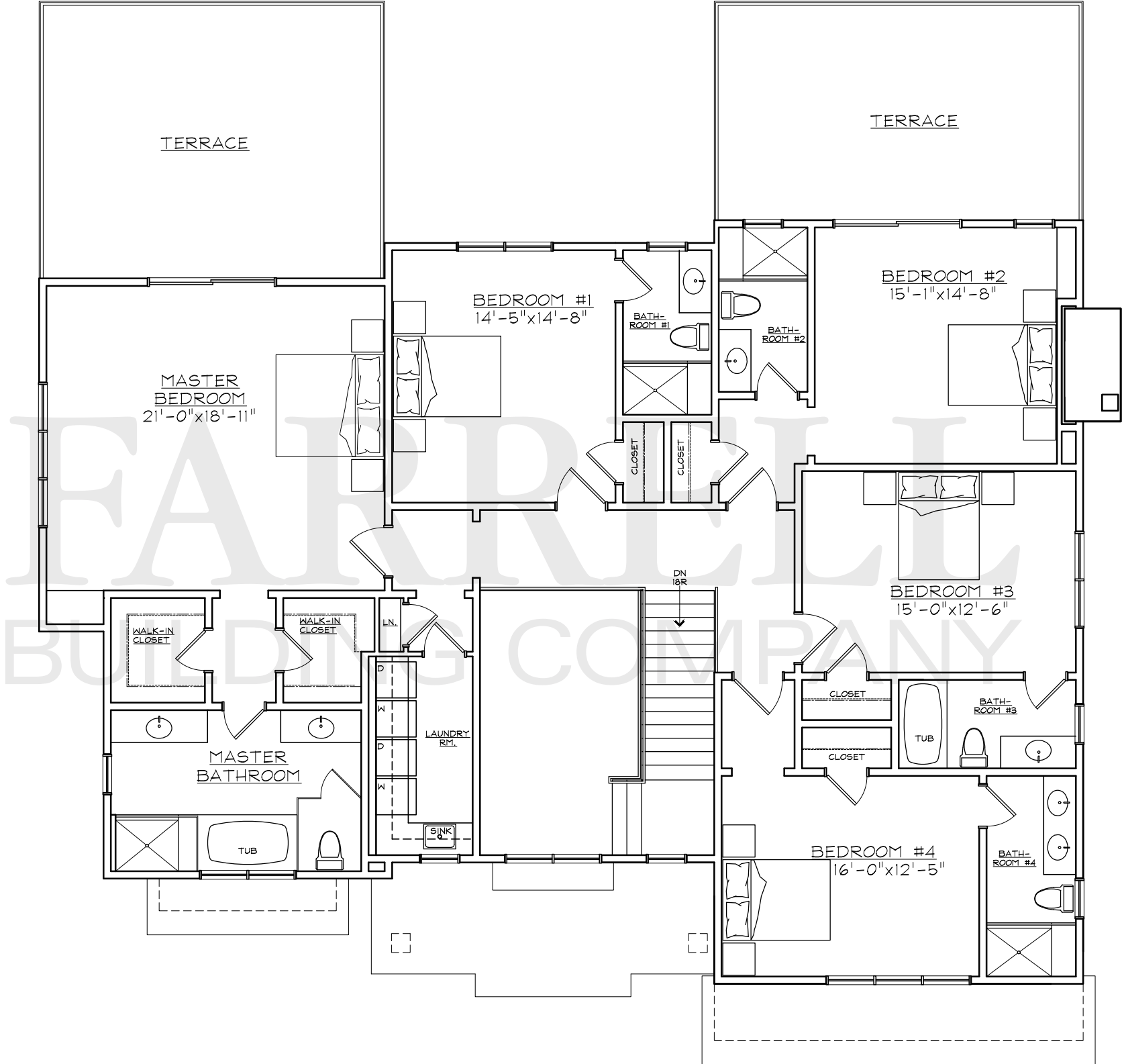
SECOND FLOOR PLAN (03-17-16) ROSES GROVE ROAD 2,366 SQ. FT.
