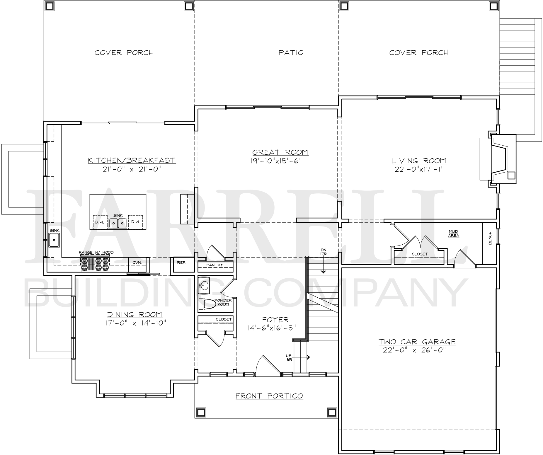
FIRST FLOOR PLAN (03-17-16)
