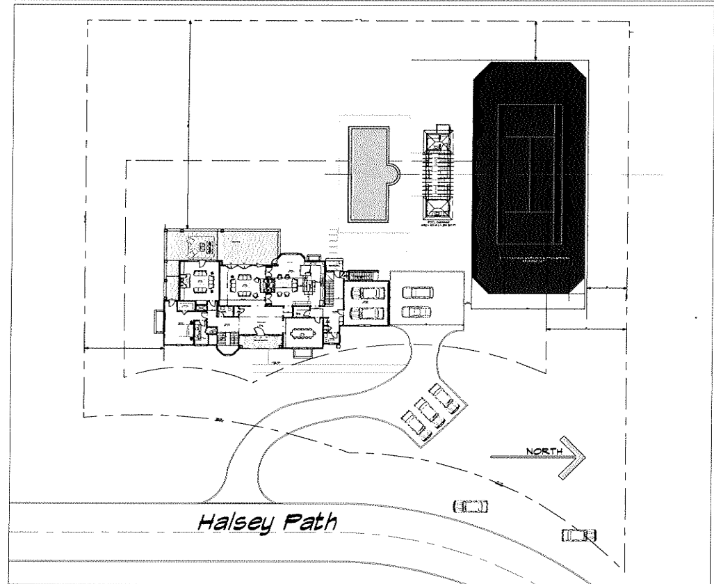
Site Plan @ 1" = 20.0' scale
