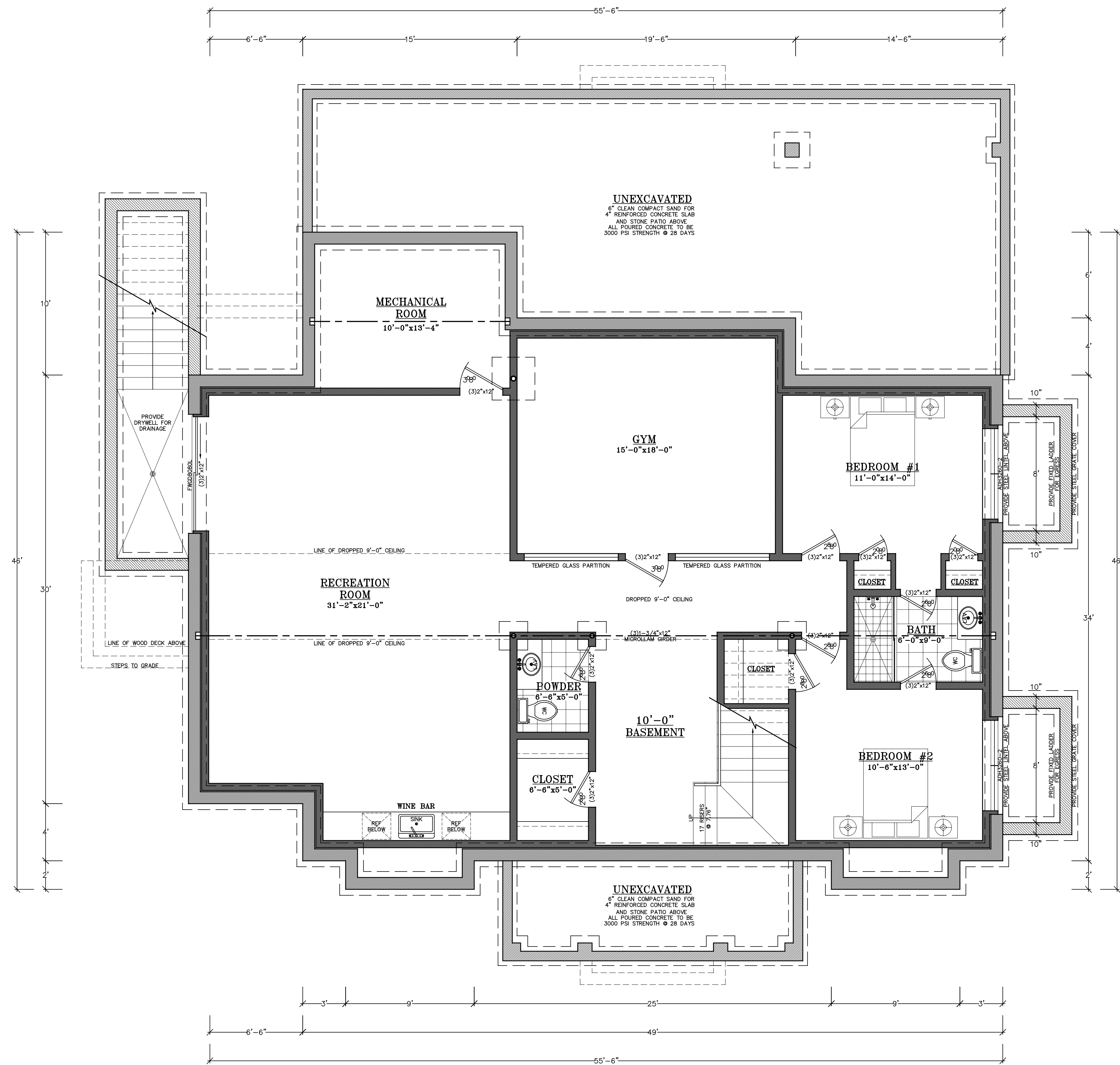
FINISHED BASEMENT PLAN LIVING AREA= 1,819 SQ.FT. SCALE: 1/4"=1'-0"
