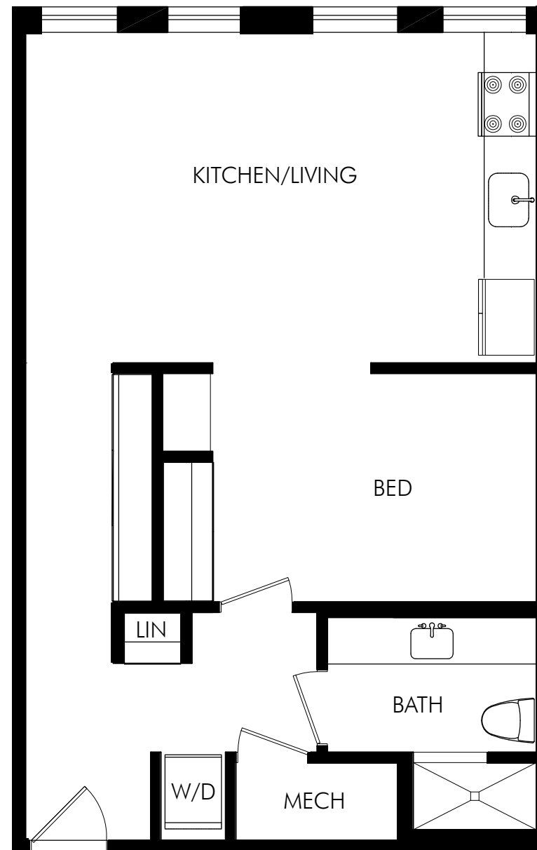
UNITS 202, 302, 402 575 square feet
