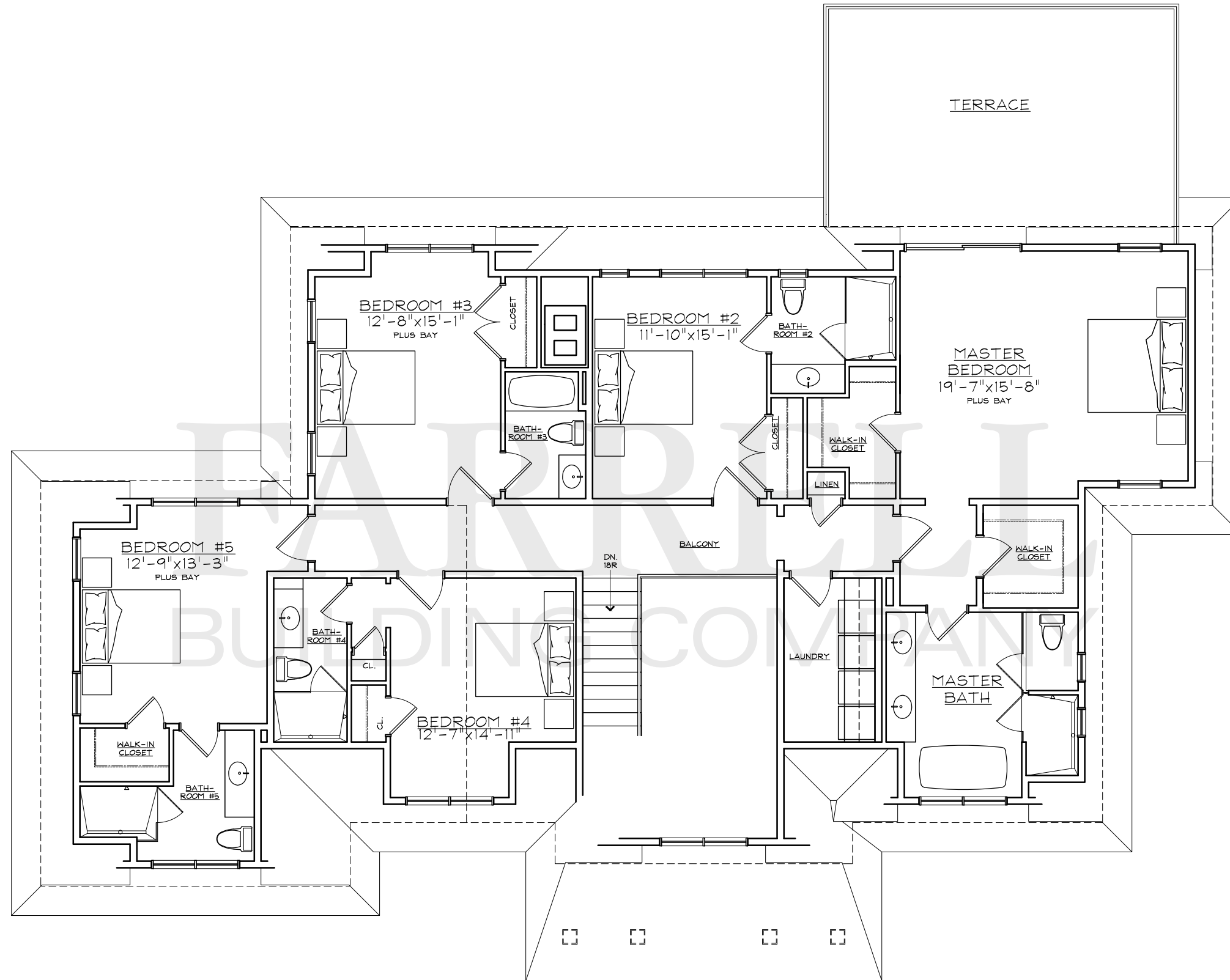
SECOND FLOOR PLAN (03-14-16)
