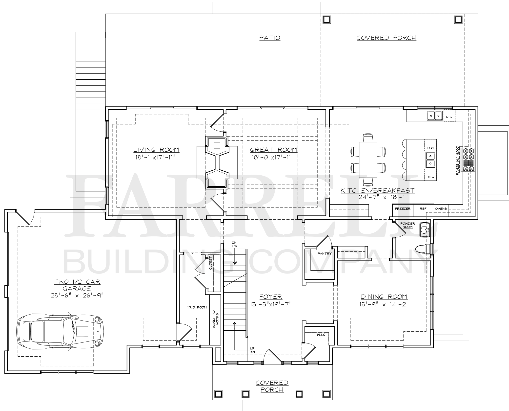
FIRST FLOOR PLAN (03-14-16)
