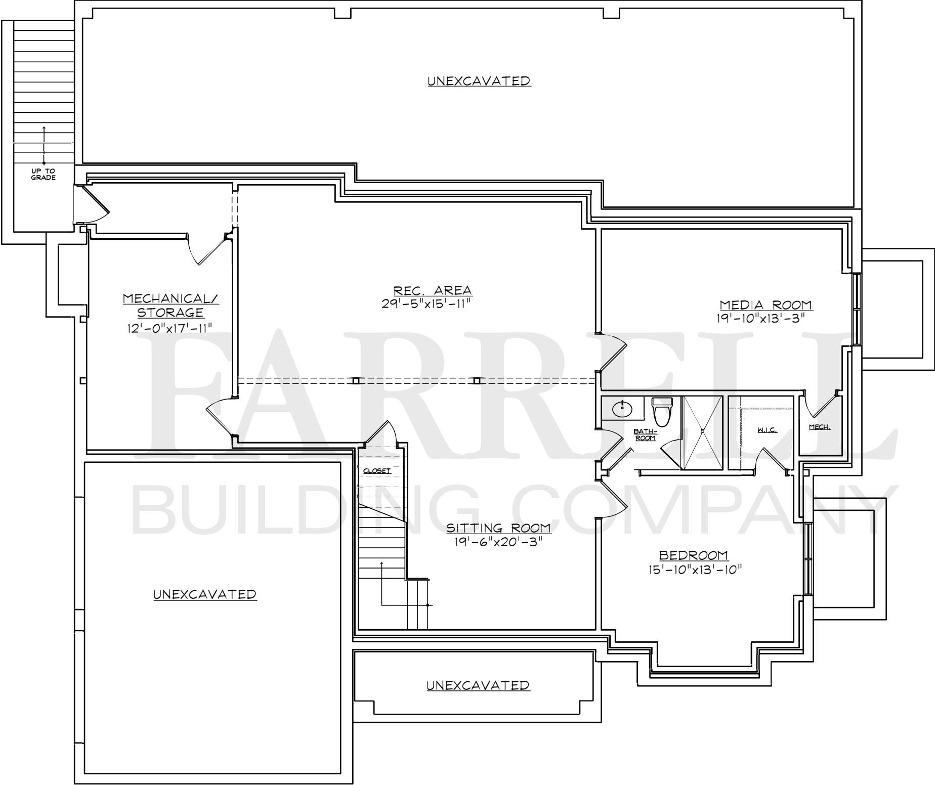
LOWER LEVEL PLAN (03-09-16) HANDS CREEK ROAD LOT 1 1,922 SQ.FT.
