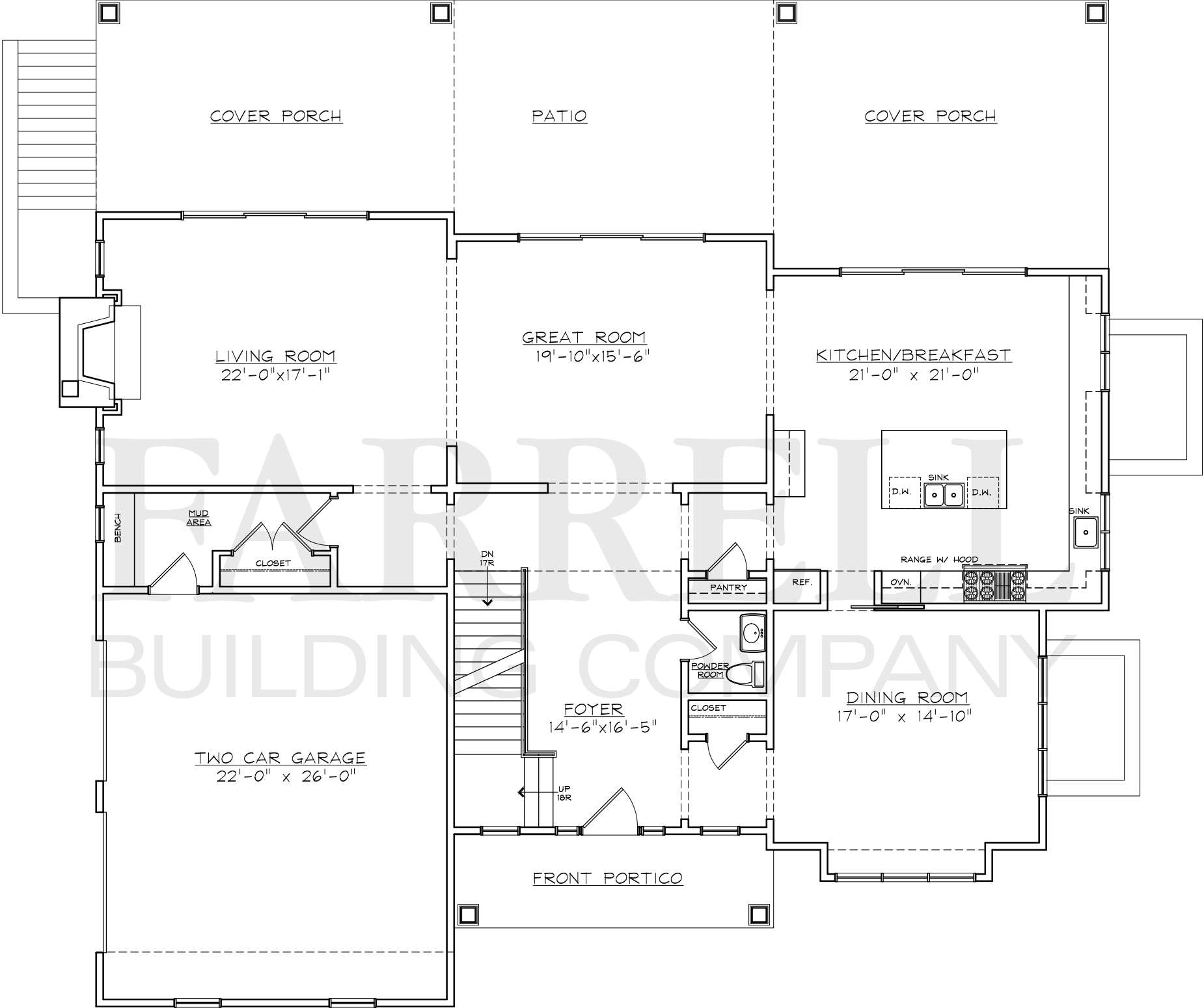
FIRST FLOOR PLAN (03-09-16)
