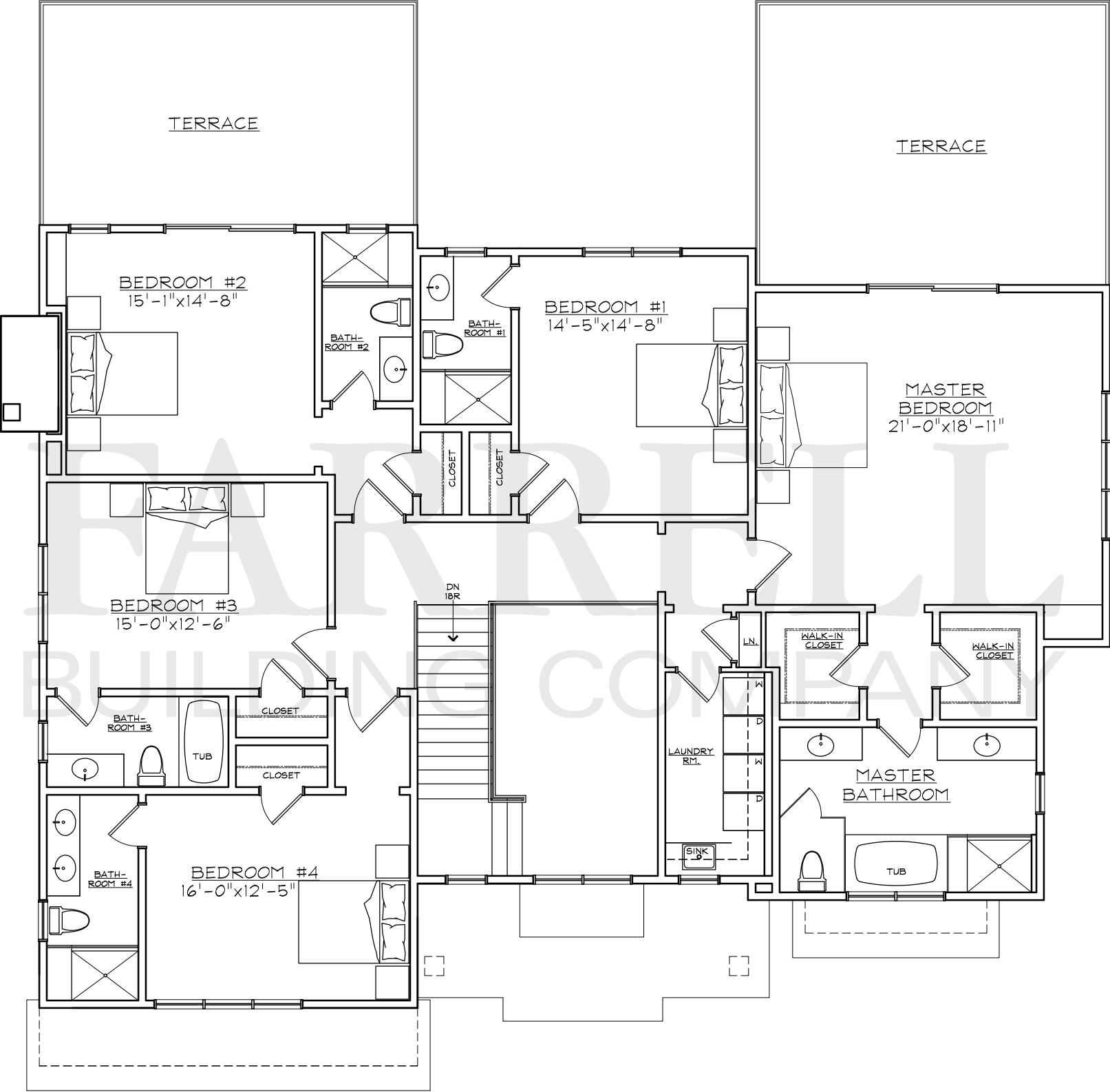
SECOND FLOOR PLAN (03-09-16) HANDS CREEK ROAD LOT 1 2,366 SQ. FT.
