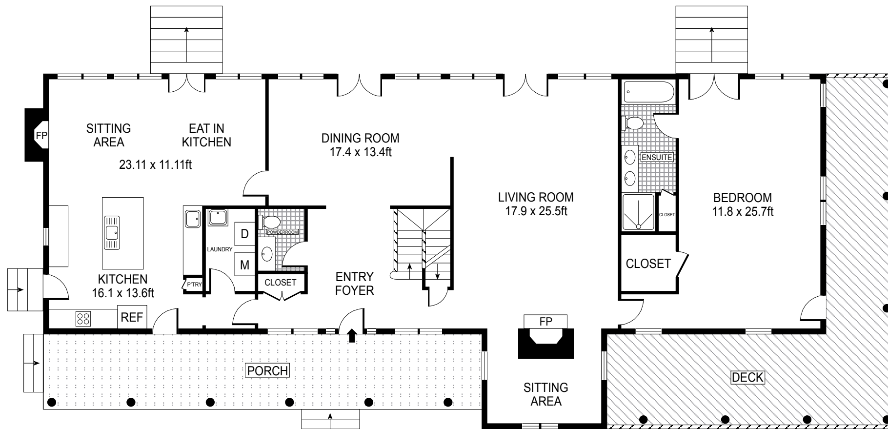
FIRST FLOOR
