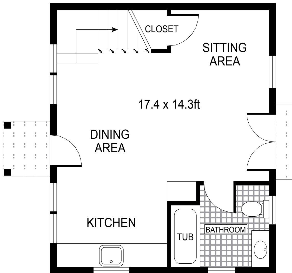
FIRST FLOOR
