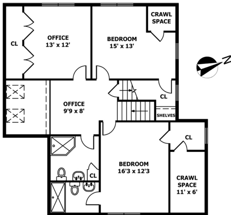
SECOND FLOOR
