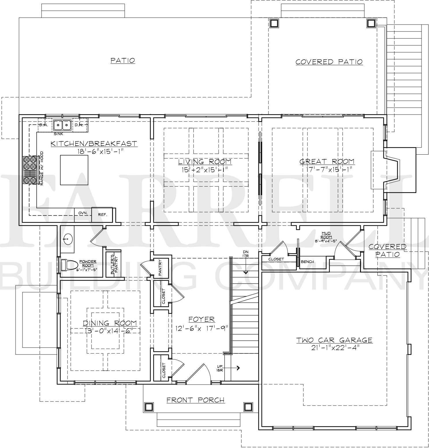
FIRST FLOOR PLAN (02-07-17) WOODLAND DRIVE
