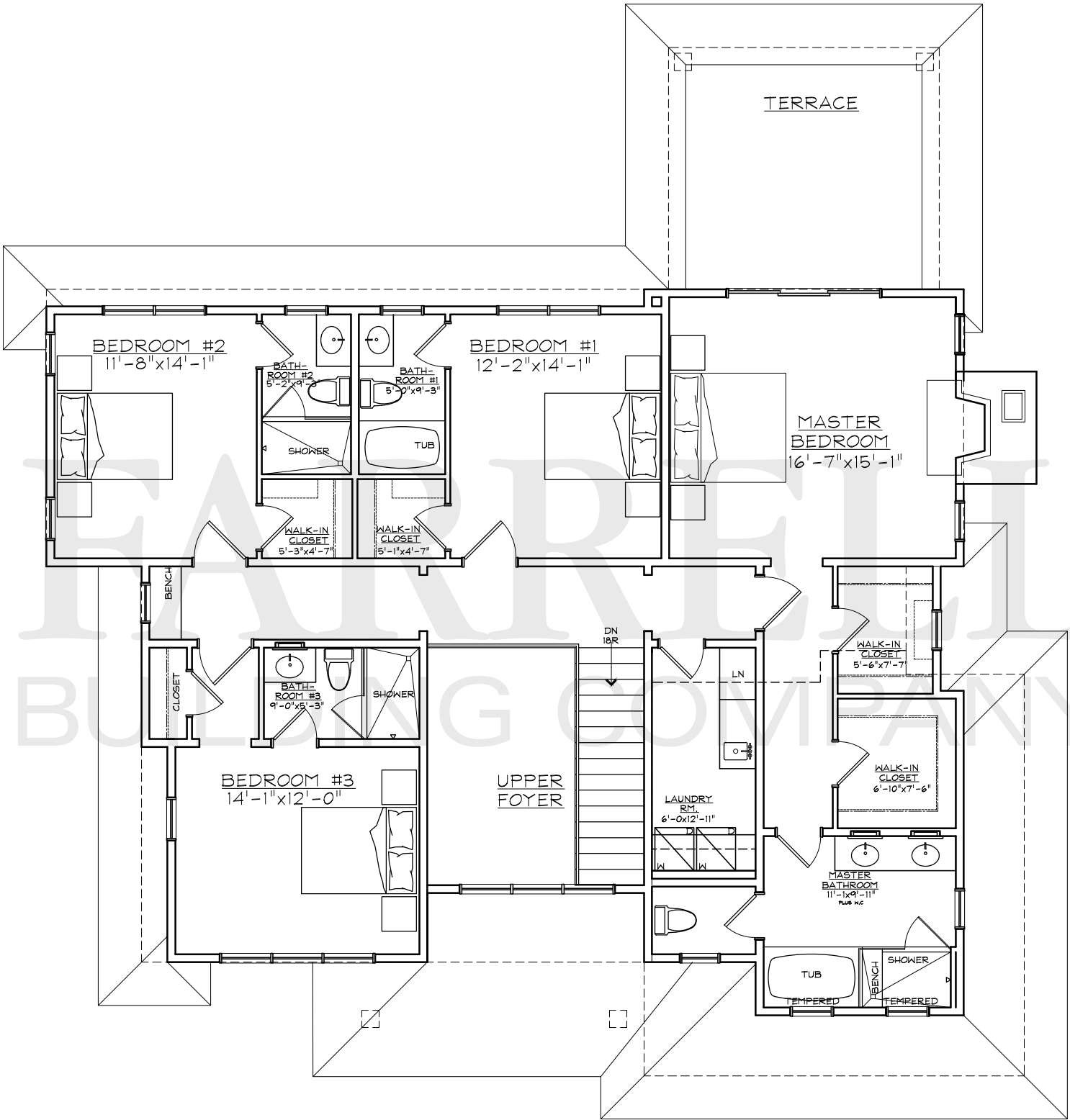
SECOND FLOOR PLAN (02-07-17) WOODLAND DRIVE 1,688 SQ. FT.
