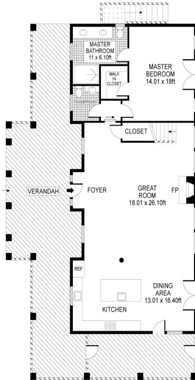
FIRST FLOOR
