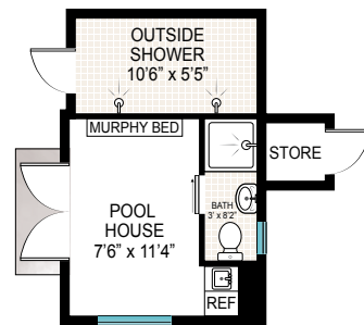
POOL HOUSE PLAN
