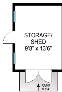
SHED PLAN
