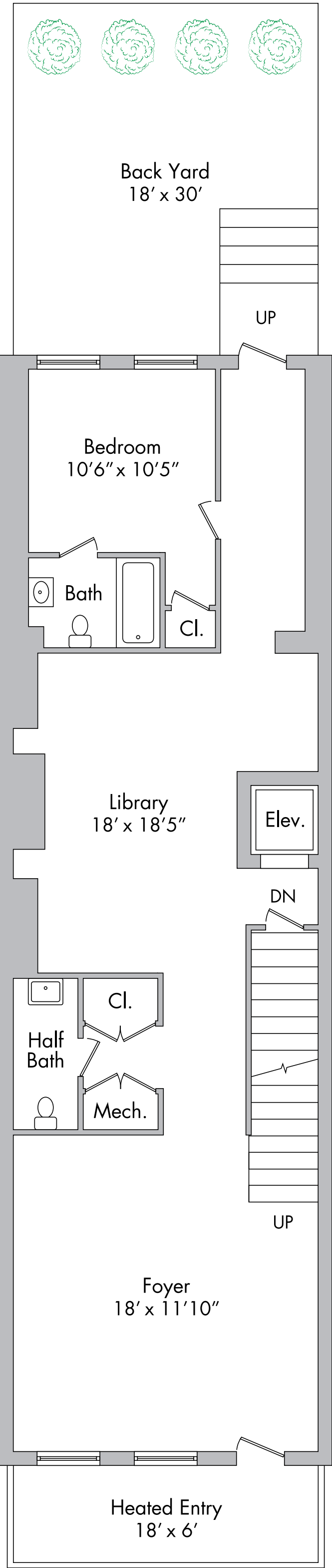
1 ST FLOOR
