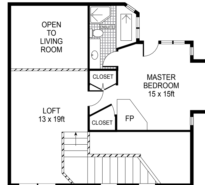
SECOND FLOOR
