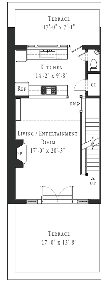
FOURTH FLOOR 8'-0" CEILING HEIGHT
