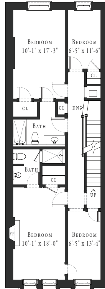
THIRD FLOOR 9'-6" CEILING HEIGHT
