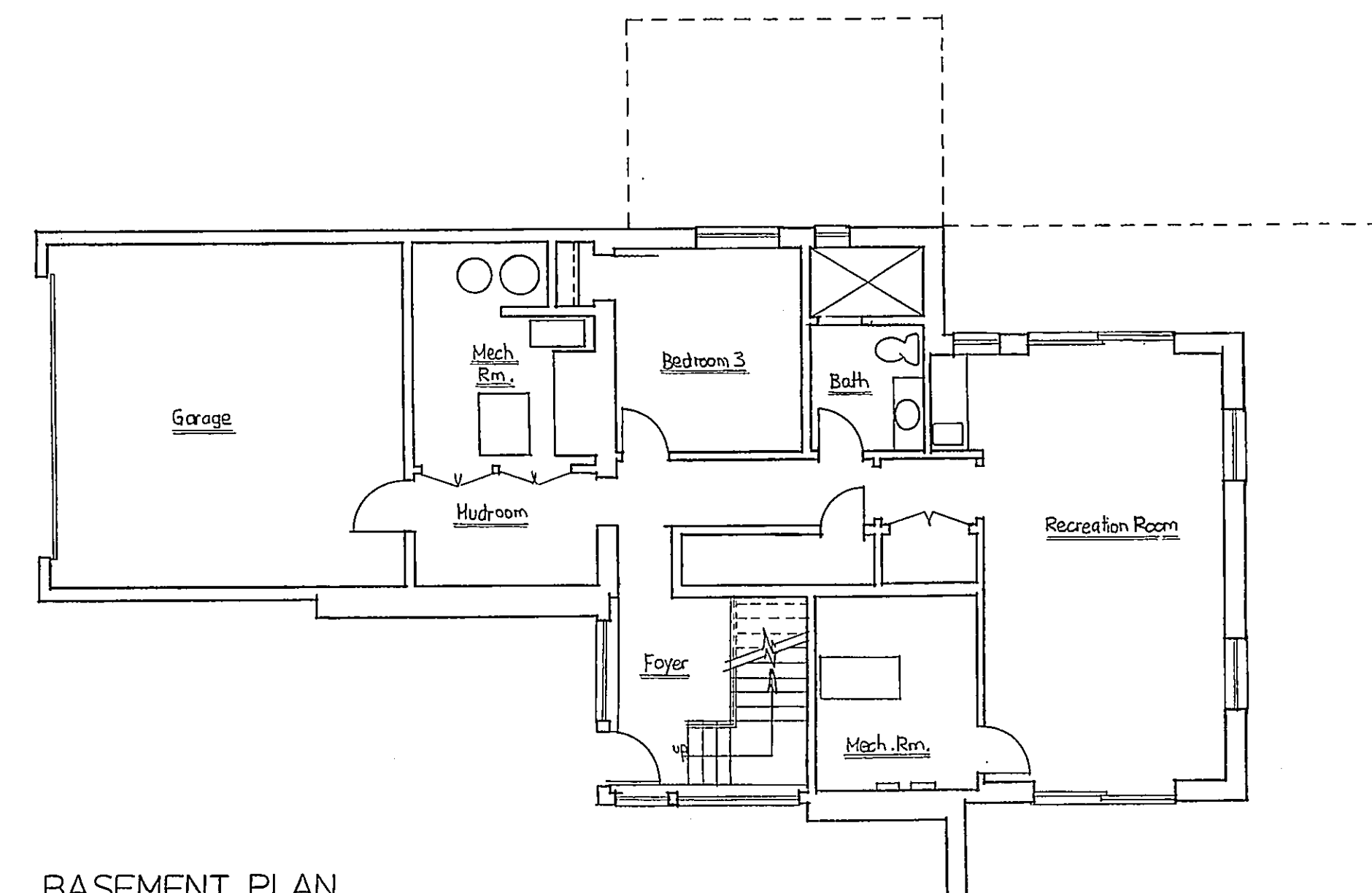
BASEMENT PLAN
