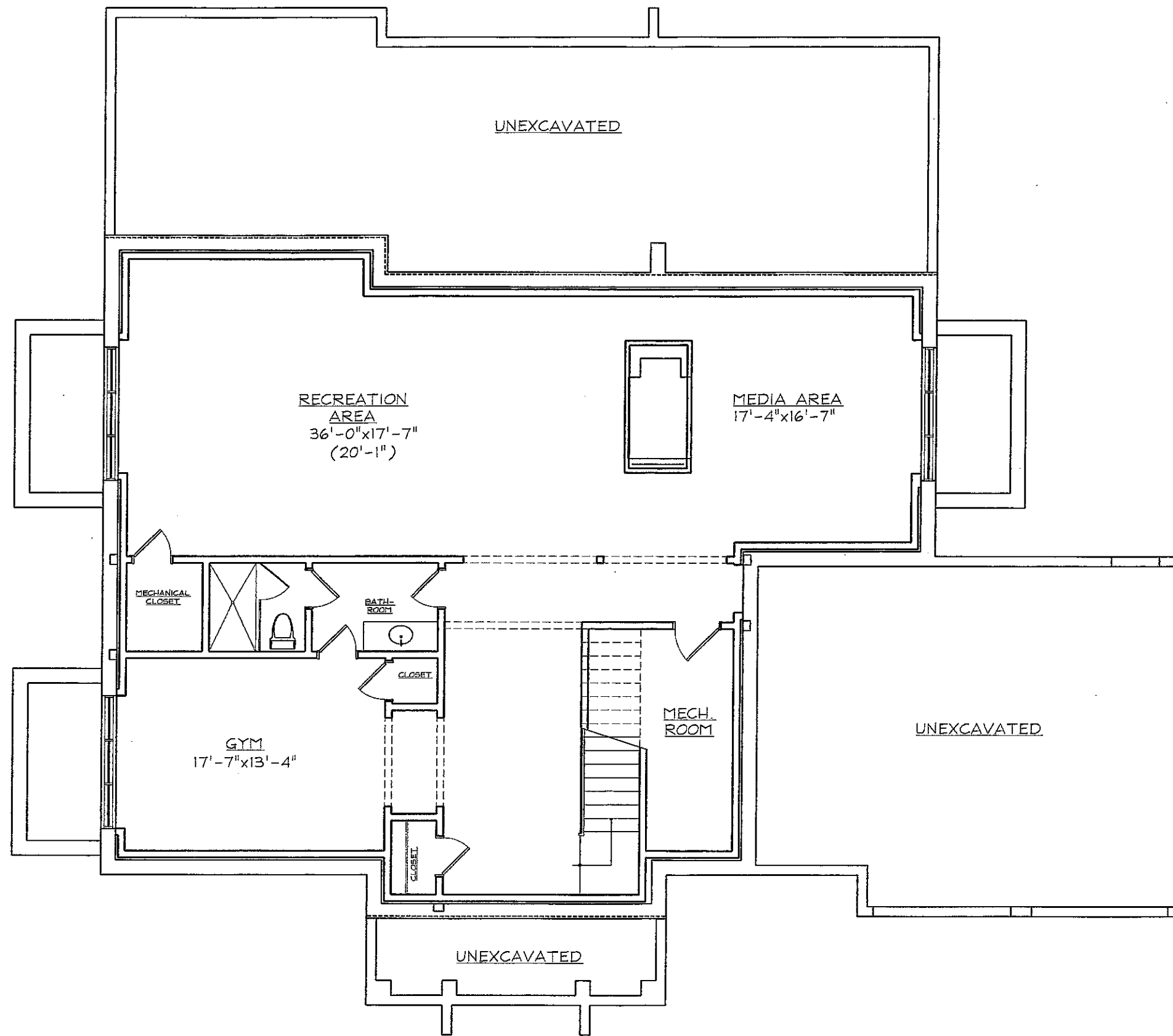
BASEMENT PLAN 52 CROSS HIGHWAY 1,844 SQ. FT.
