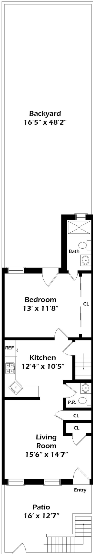
Ground Floor
