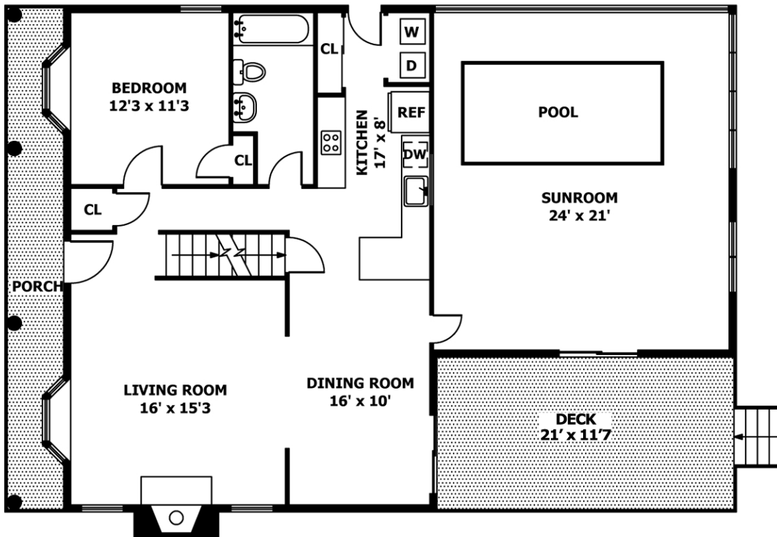
FIRST FLOOR
