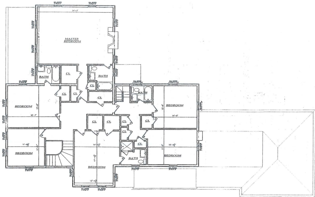
Existing Second Floor Plan SCALE: 1/4" = 1'-0"
