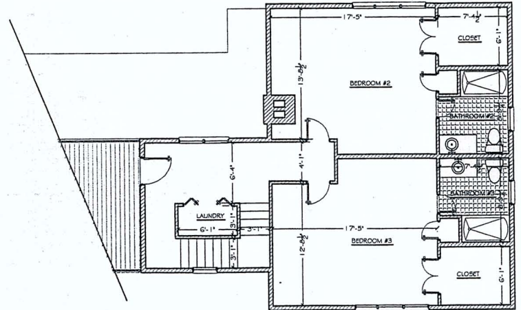
2 SECOND FLOOR PLAN SCALE: 1/4" = 1'-0"
