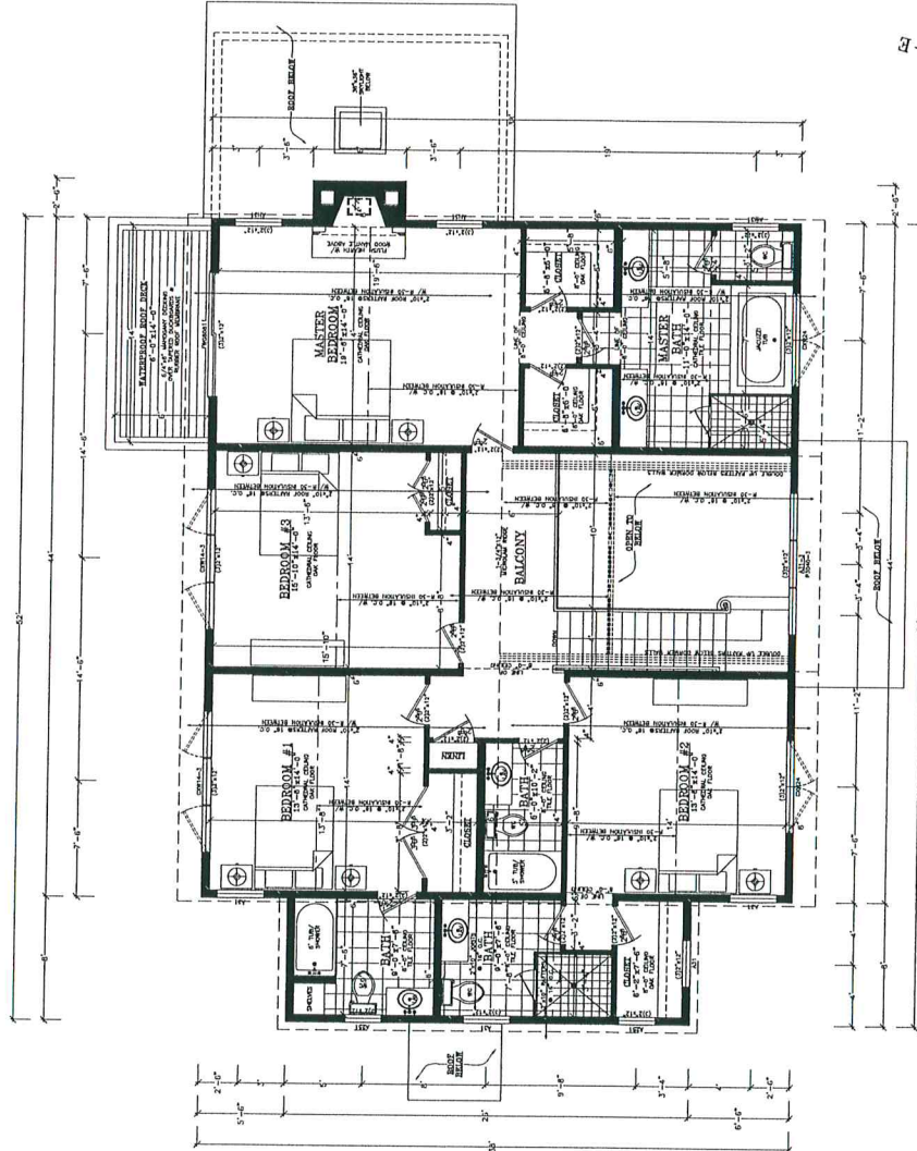
SECOND FLOOR PLAN LIVING AREA = 1,644 SQ. FT. DECK AREA = 64 SQ. FT. SCALE: 1/4" = 1'-0"
