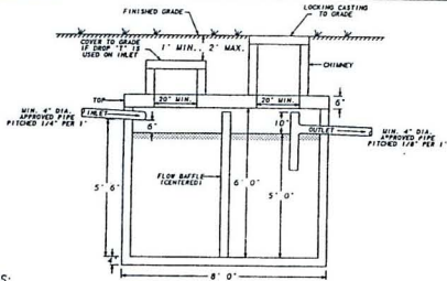
TYPICAL CYLINDRICAL 1,500 GALLON SEPTIC TANK WITH SLAB
