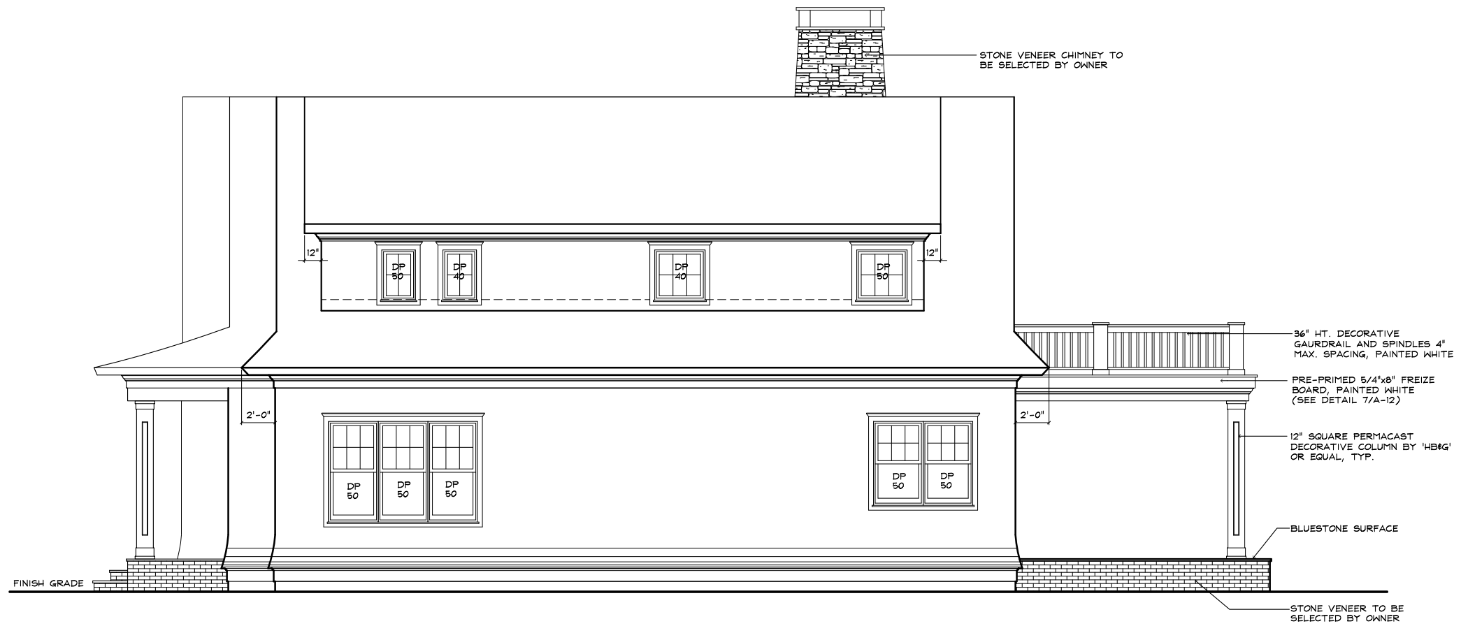
RIGHT ELEVATION PEACH FARM LANE (LOT 1)
