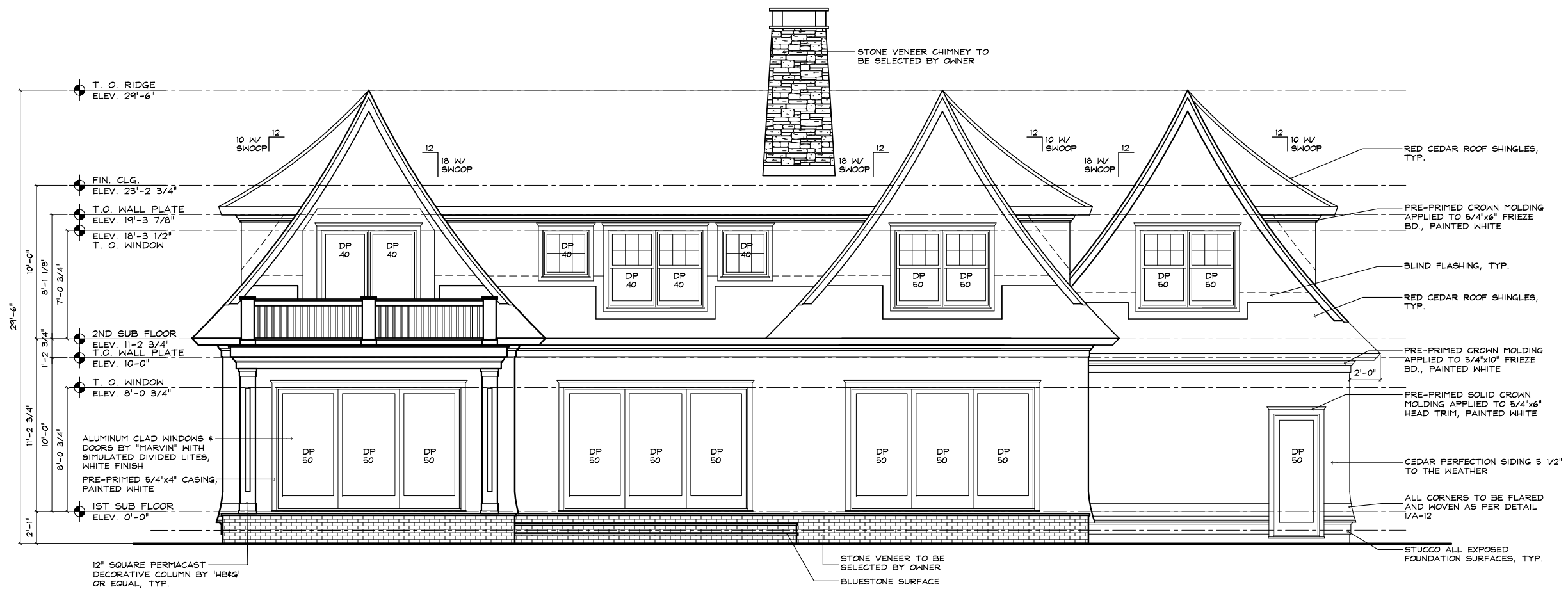
REAR ELEVATION PEACH FARM LANE (LOT 1)
