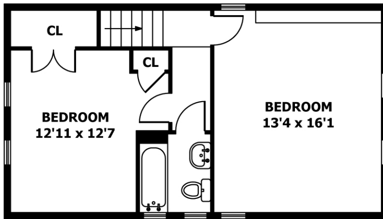
SECOND LEVEL
