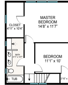
SECOND FLOOR PART 1 APARTMENT #1
