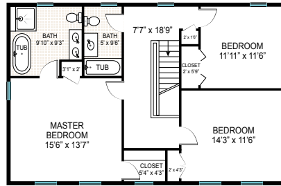
MAIN HOUSE SECOND FLOOR PART 2
