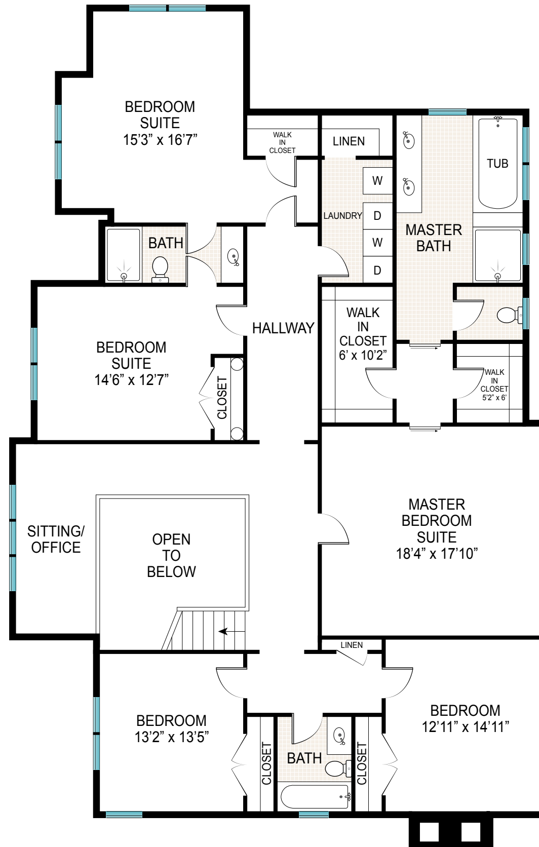
SECOND FLOOR
